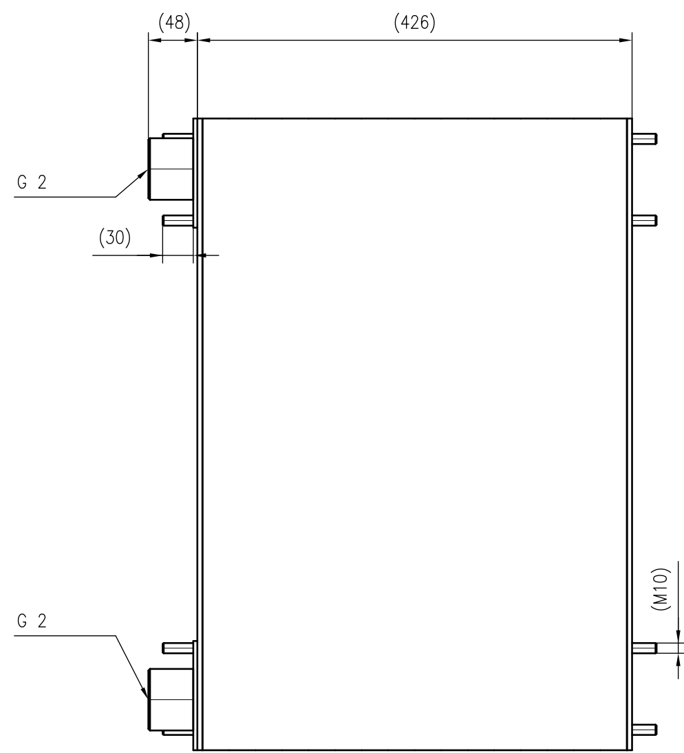
Side view
