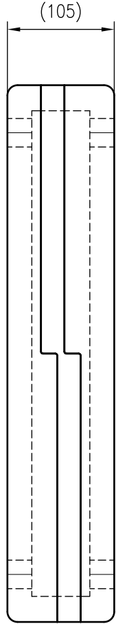
Side view
