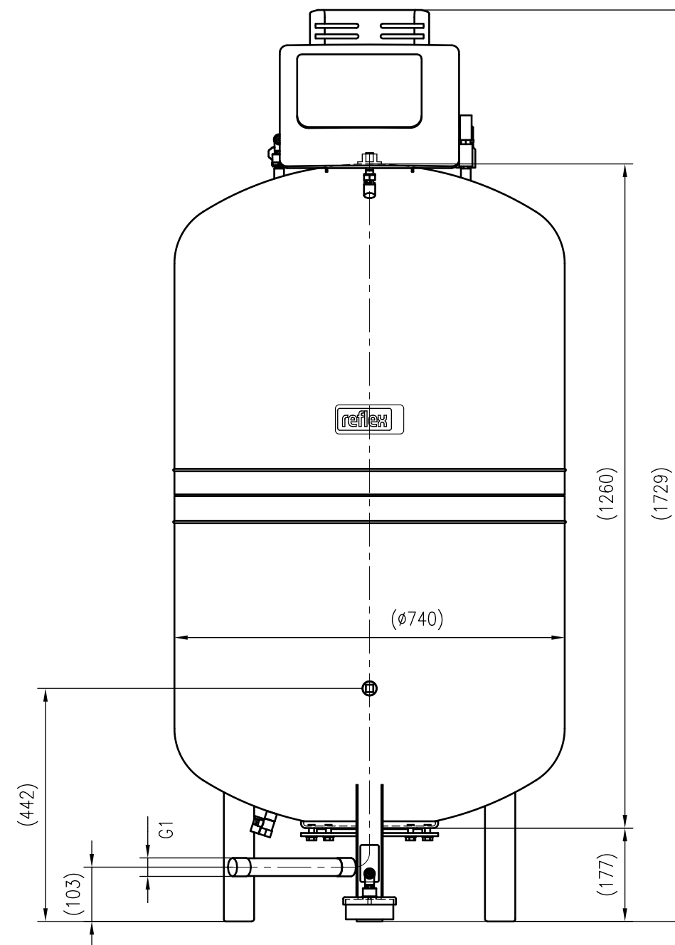
Front view
