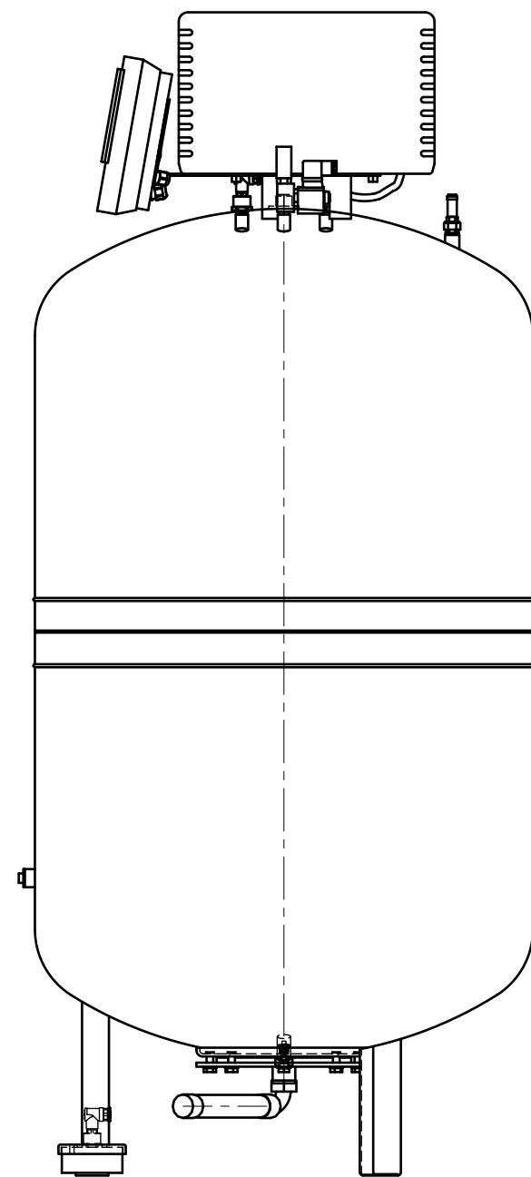
Side view
