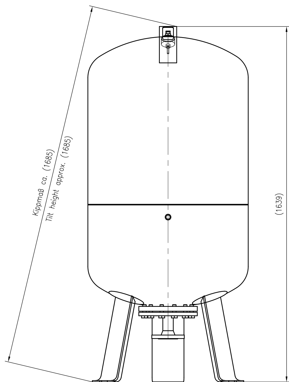
Side view
