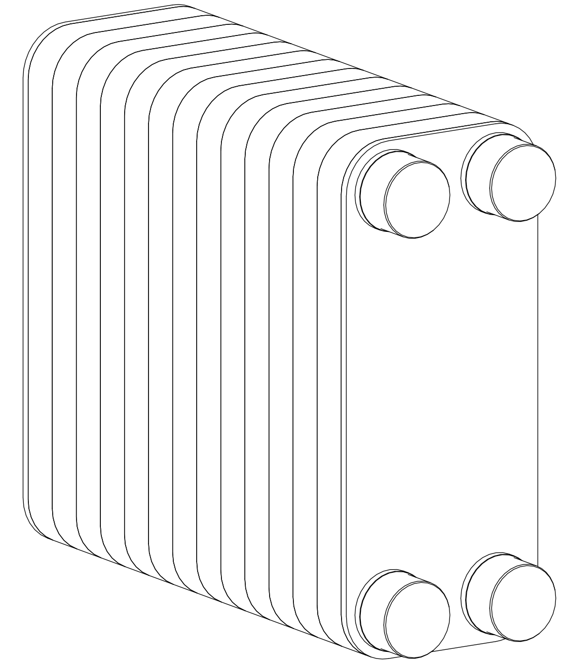
Isometric view
