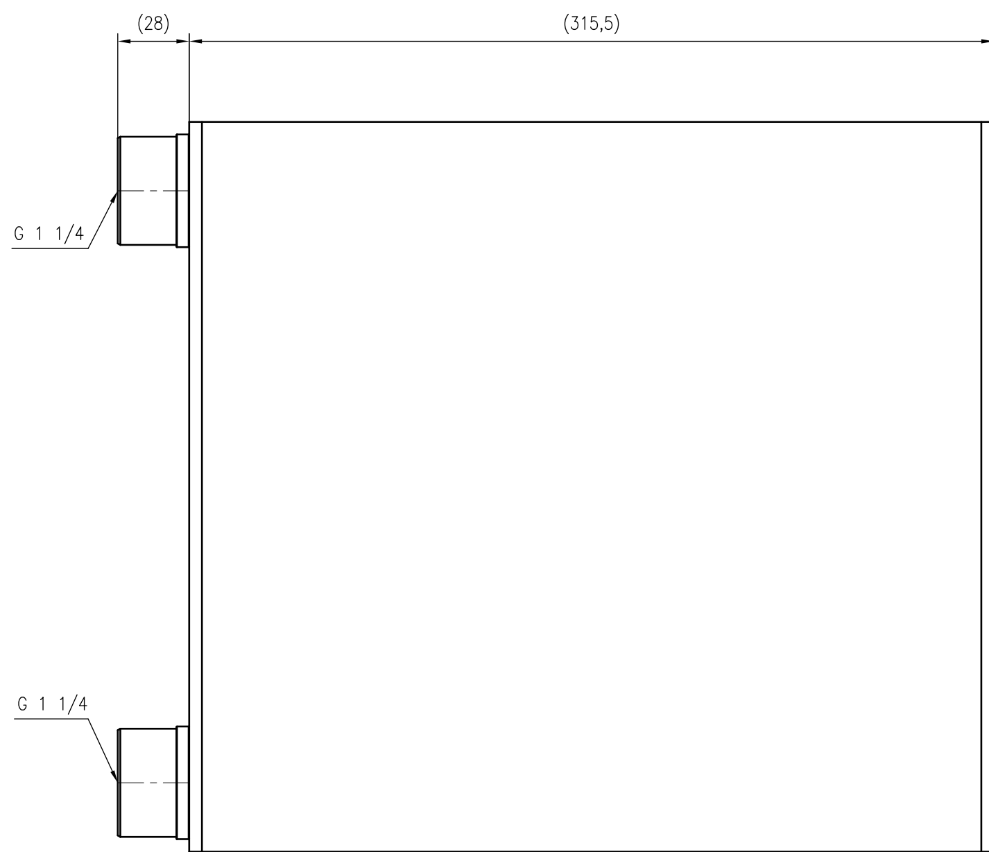
Side view
