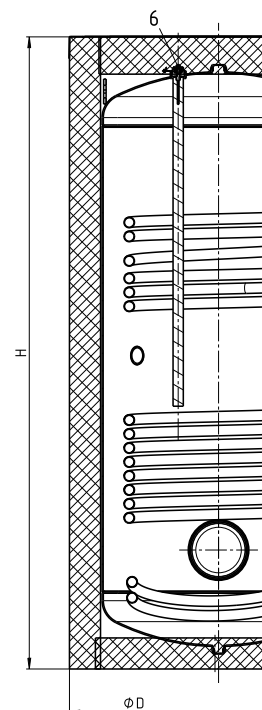
Section view B-B
