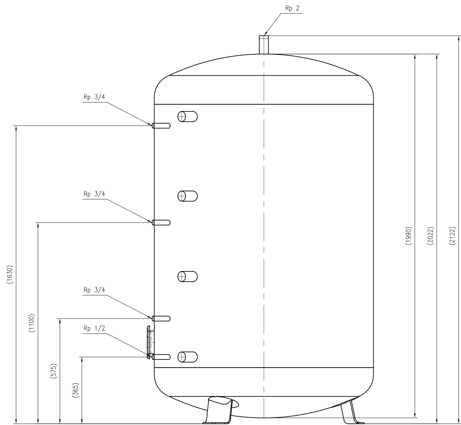
Side view
