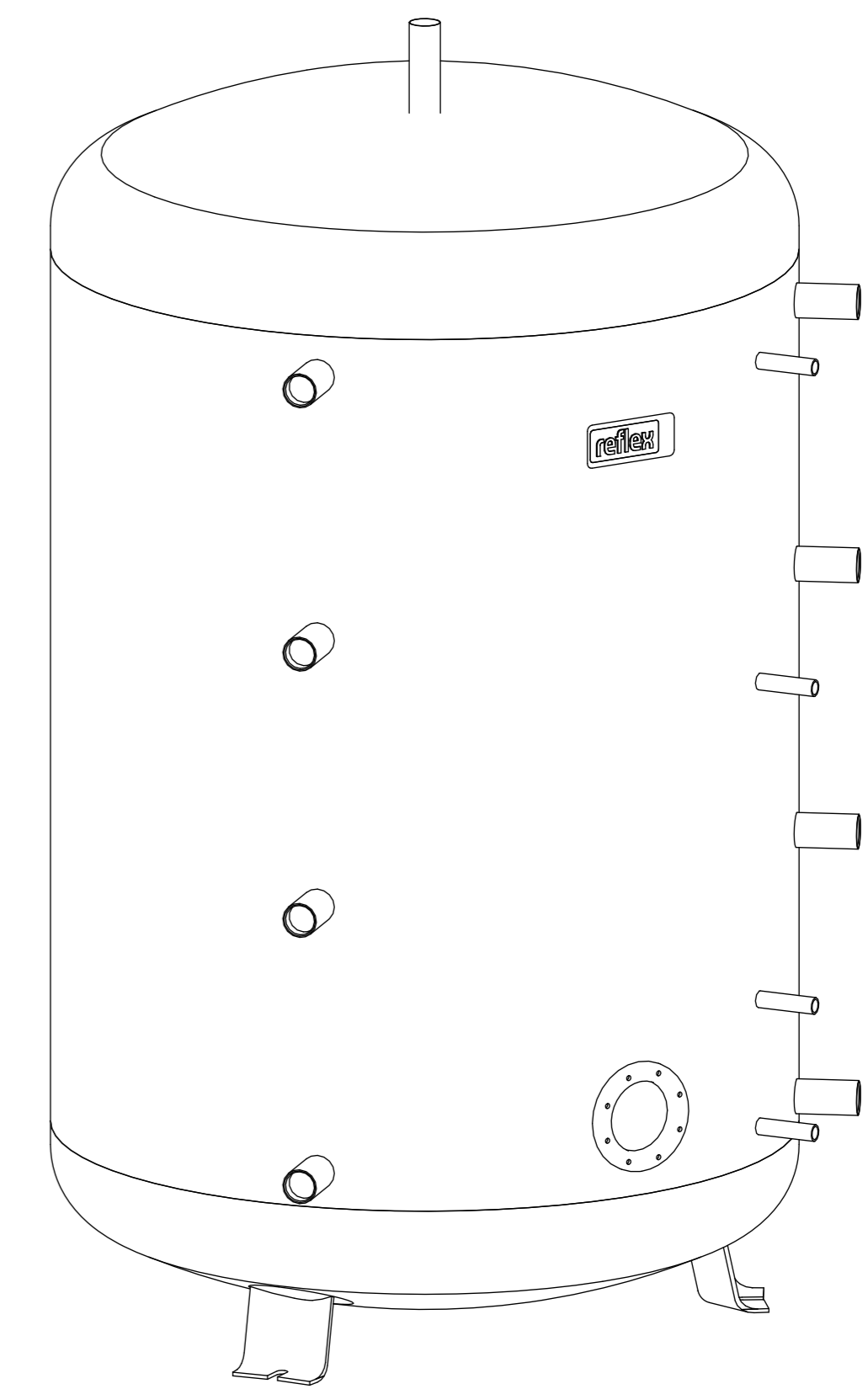
Isometric view
