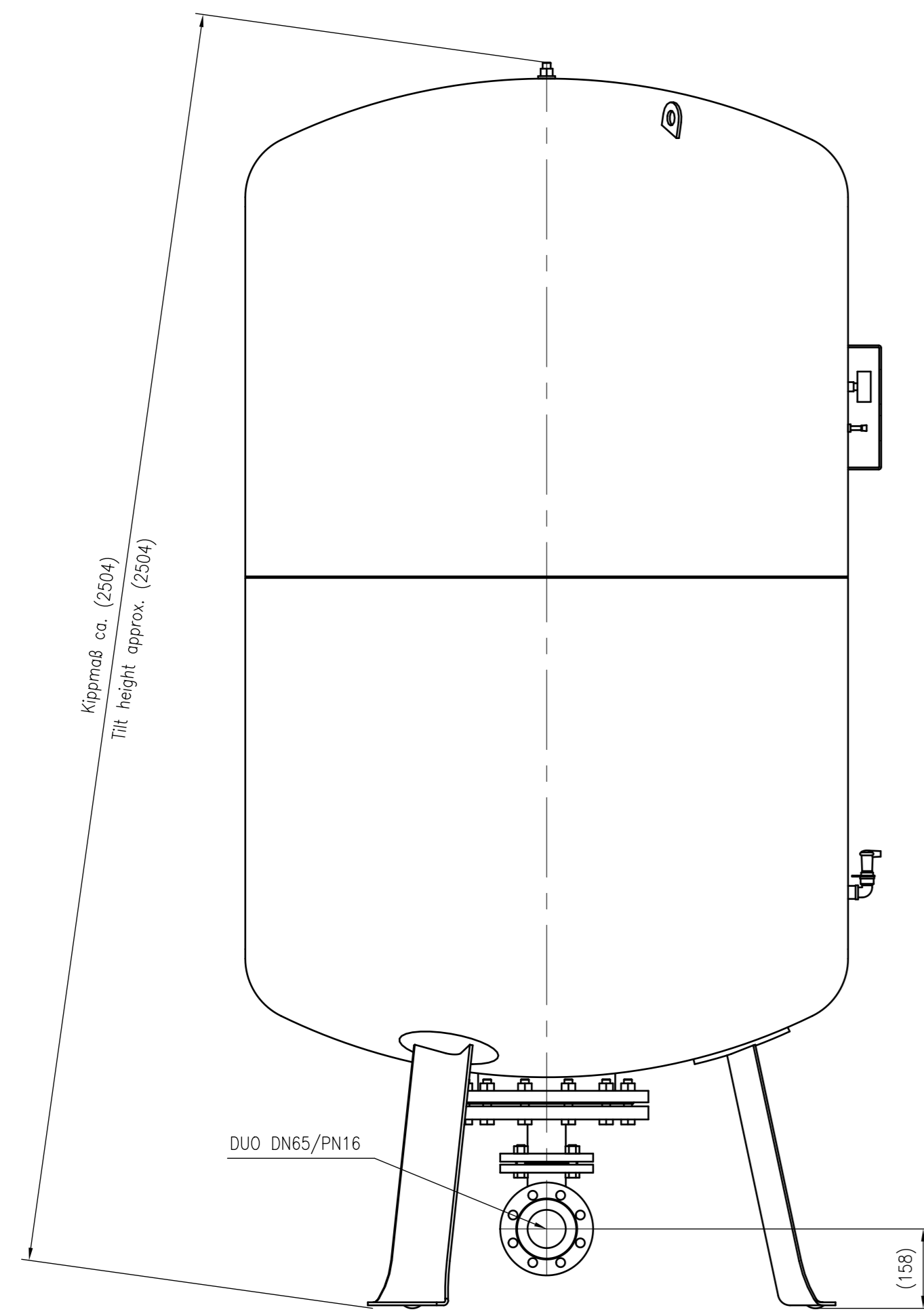
Side view
