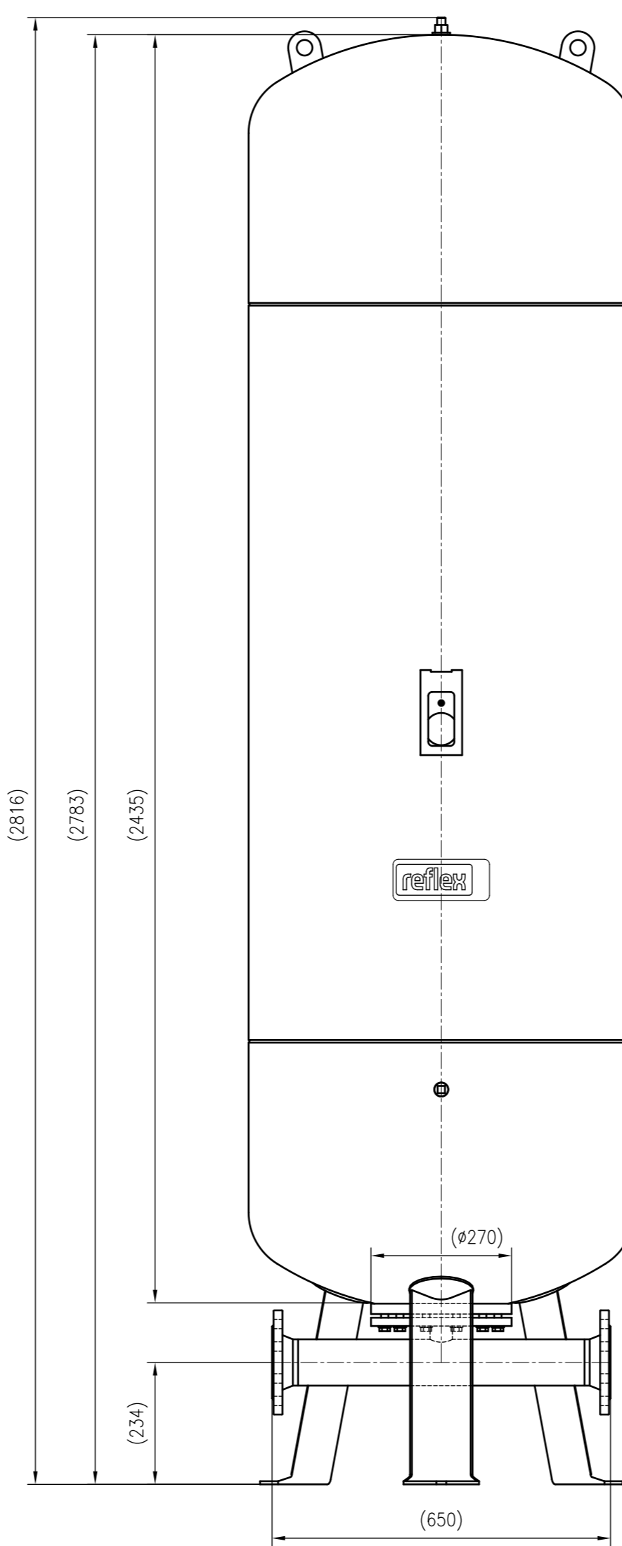
Front view
