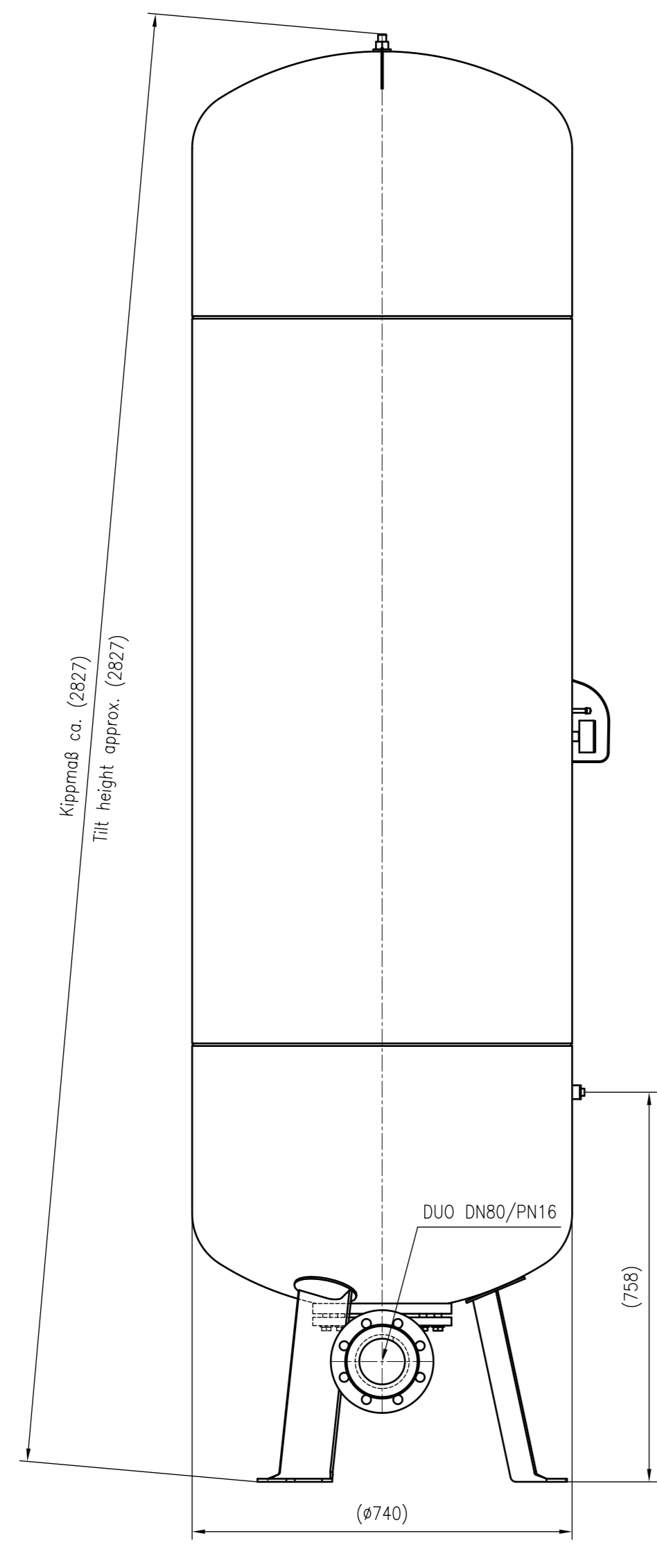
Side view
