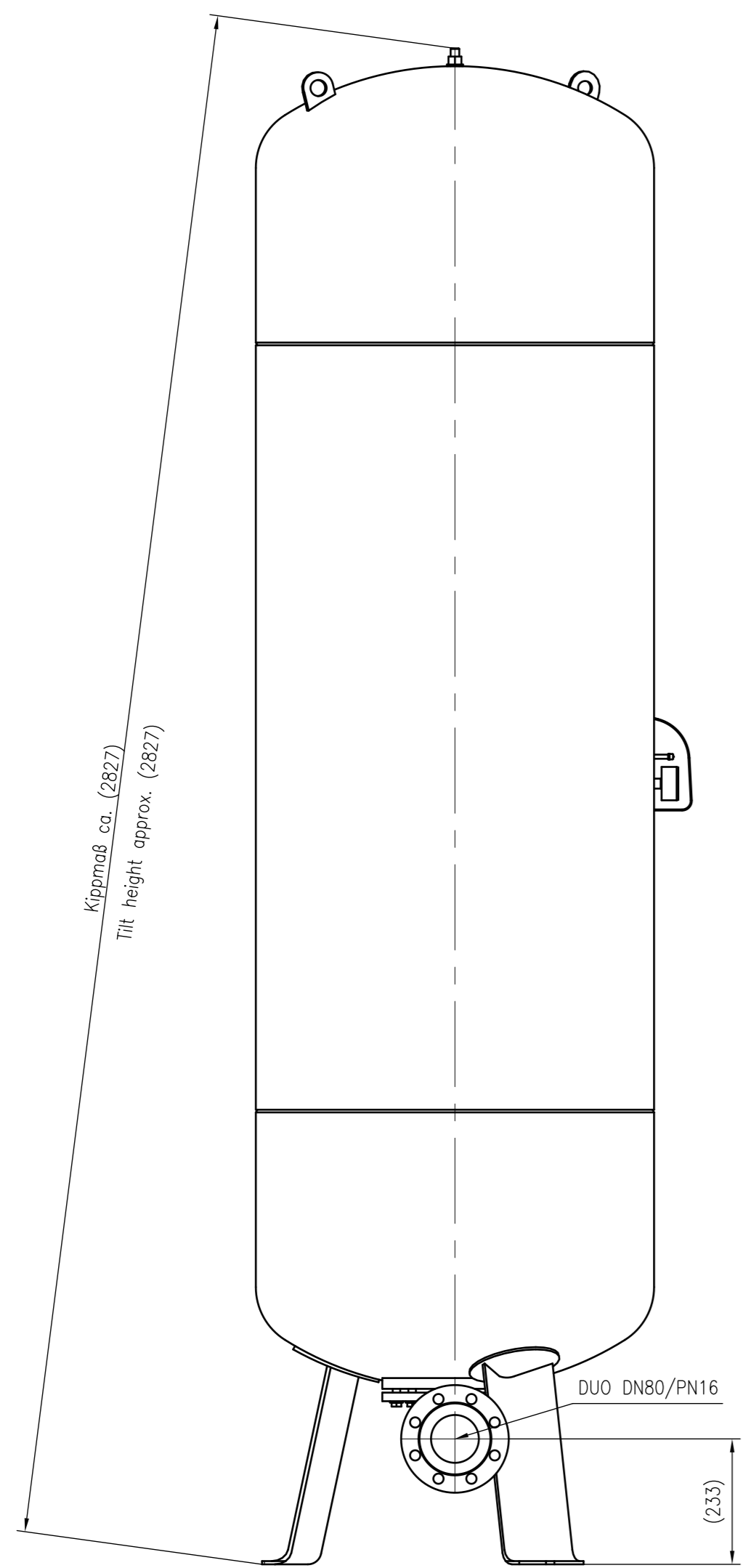
Side view
