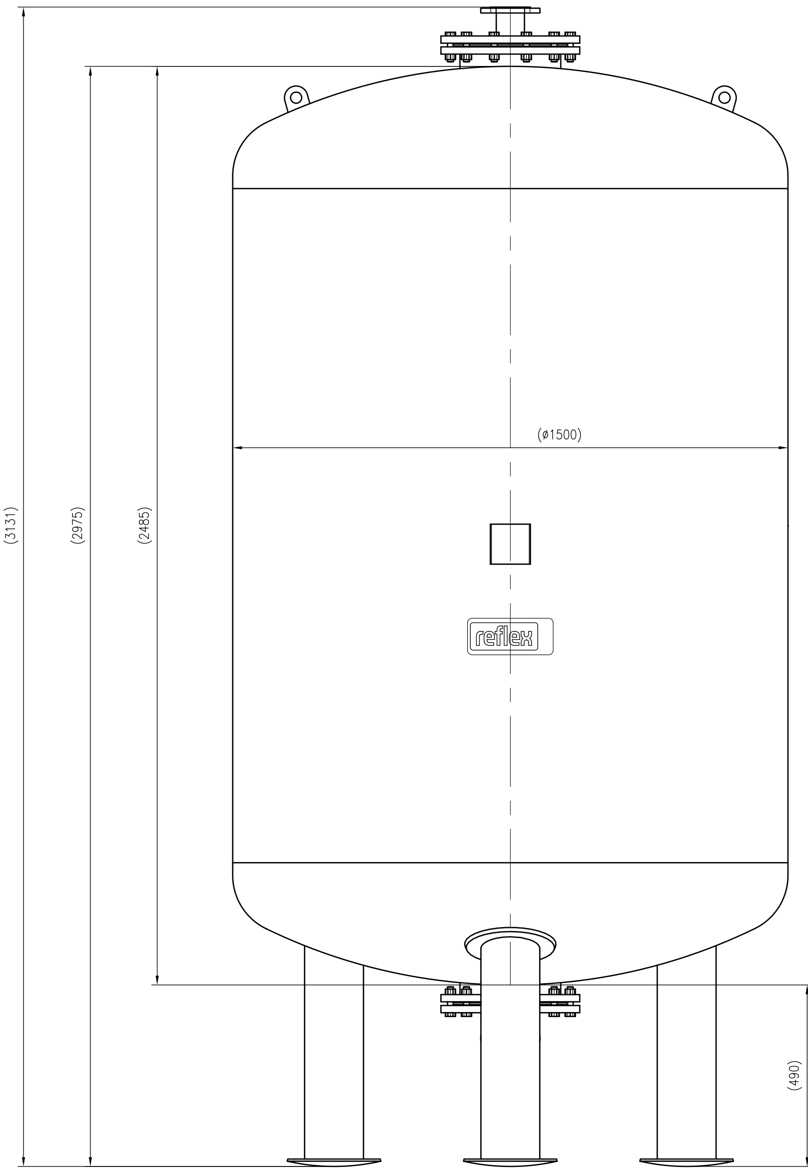
Front view
