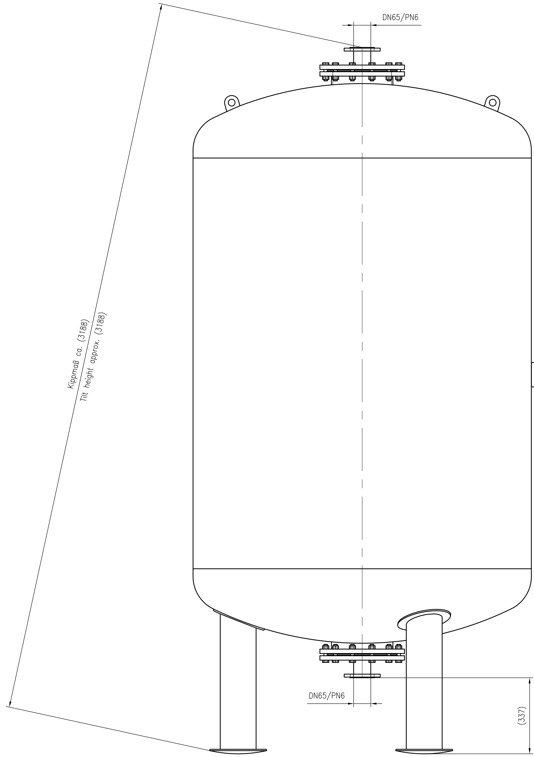
Side view
