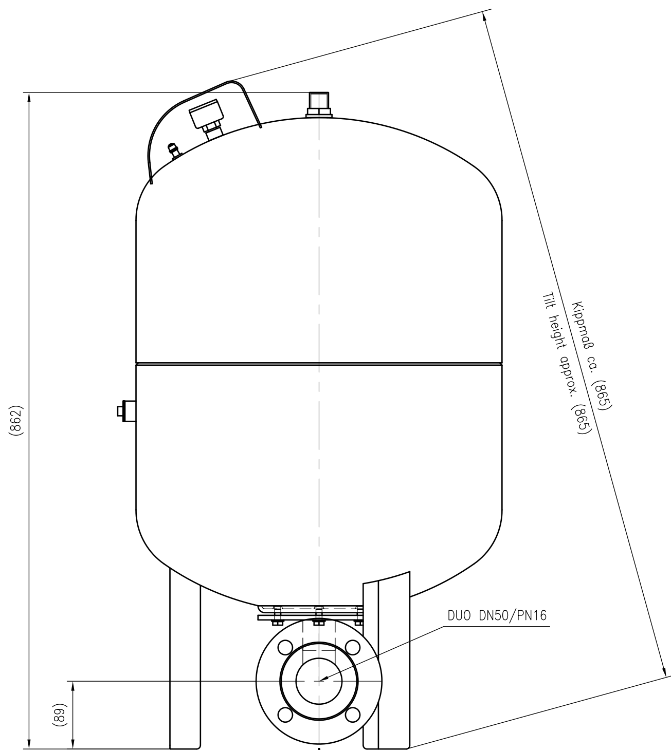
Side view
