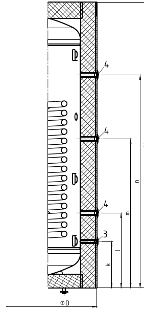
Section view C-C
