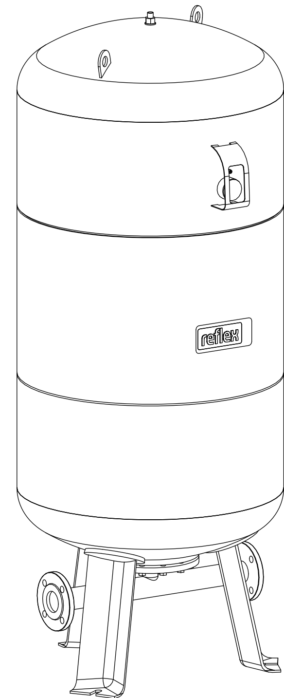
Isometric view
