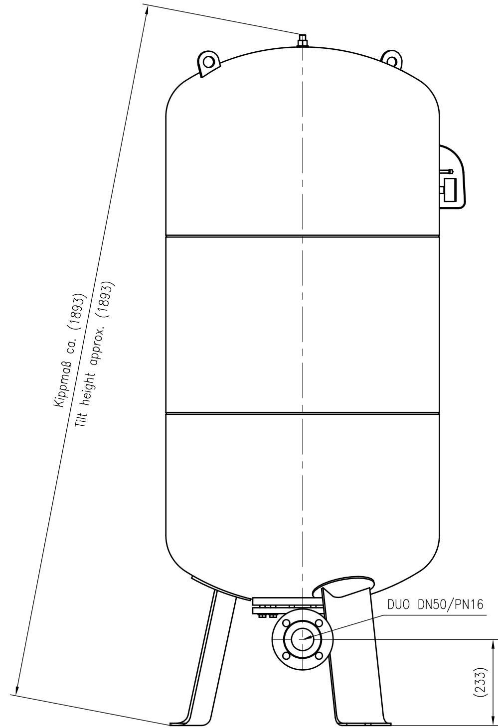
Side view
