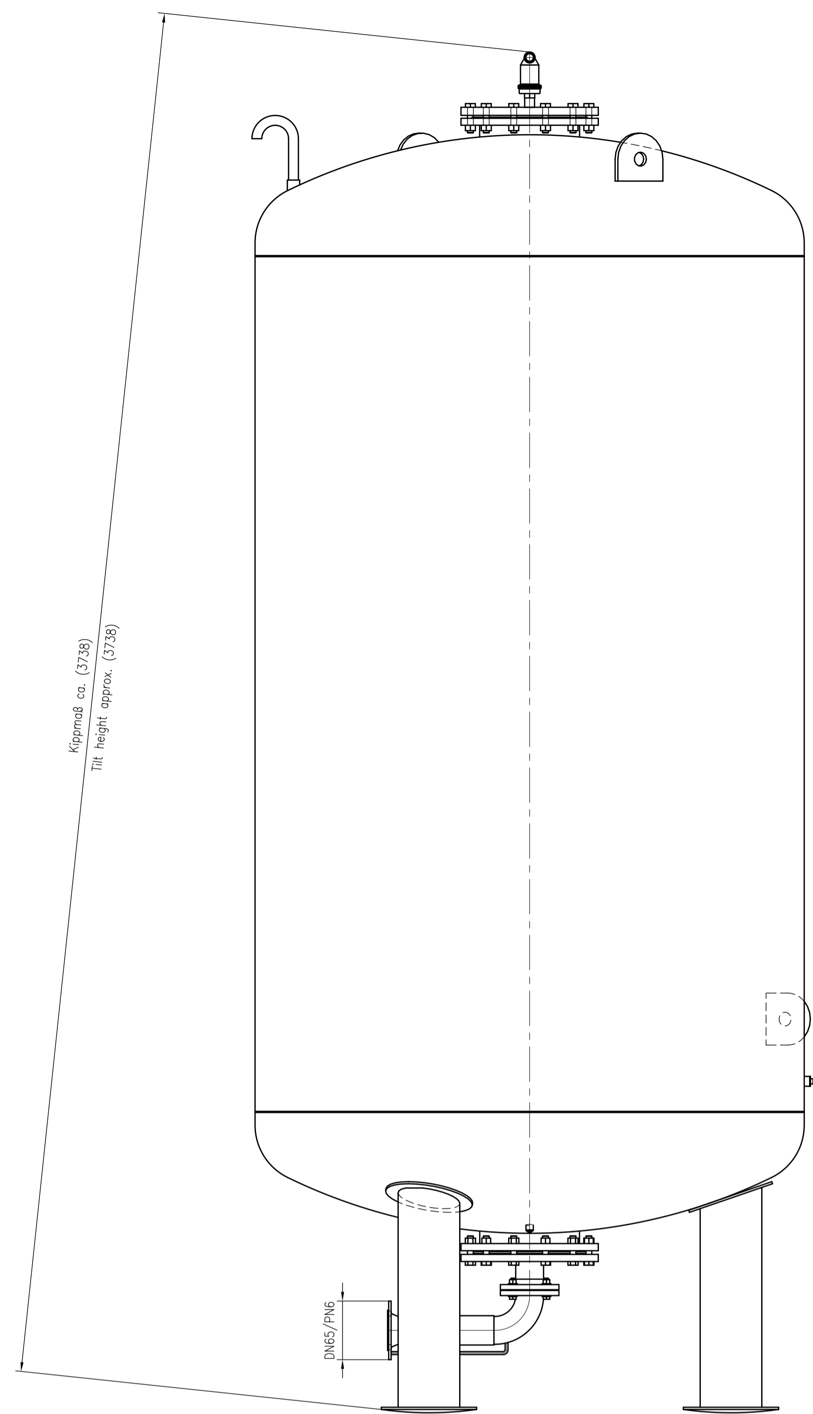
Side view
