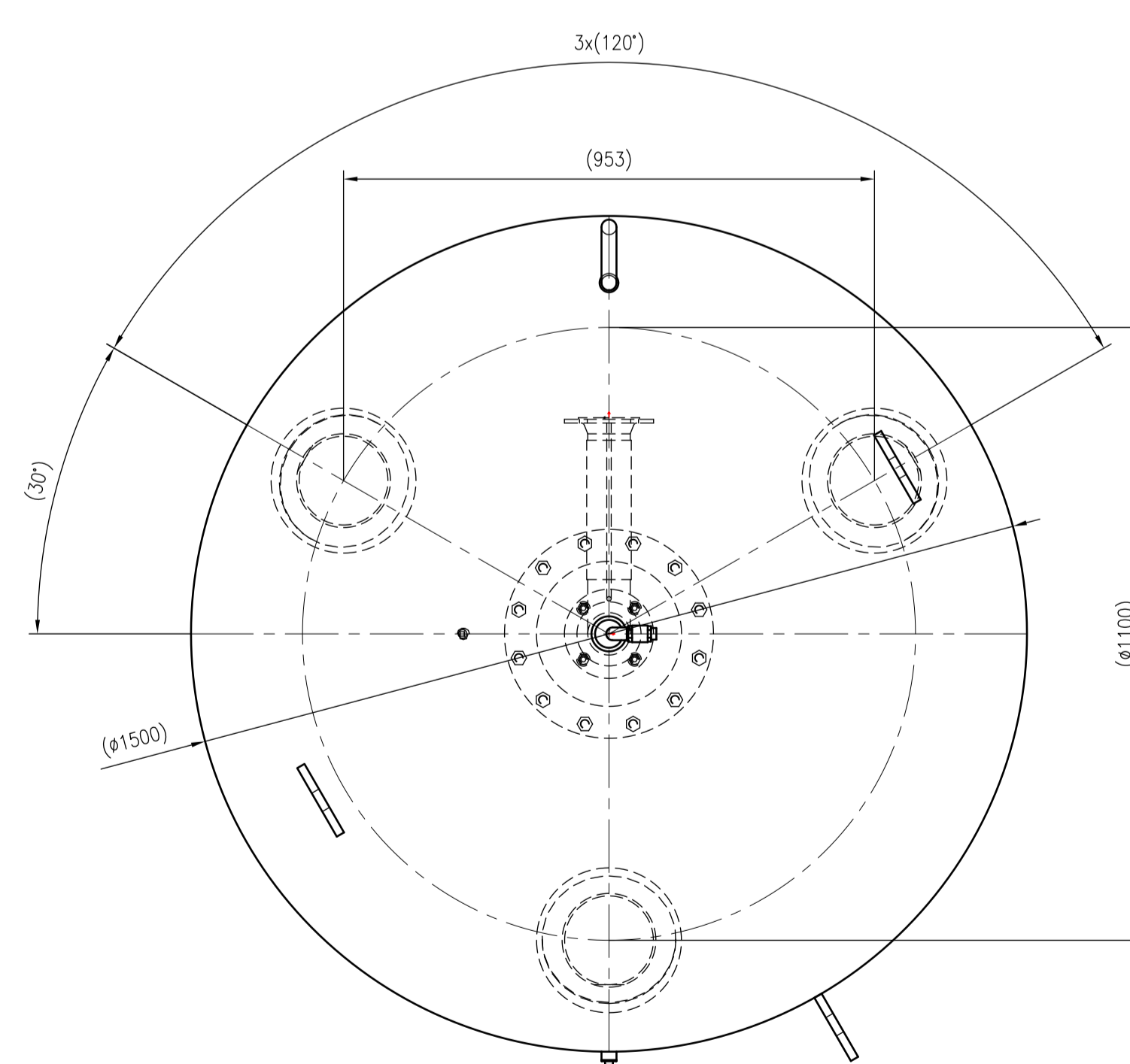
Top view
