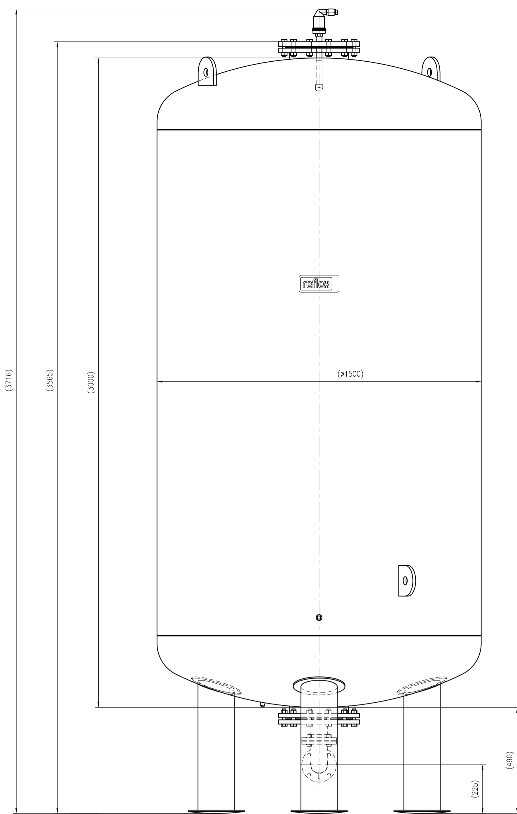
Front view
