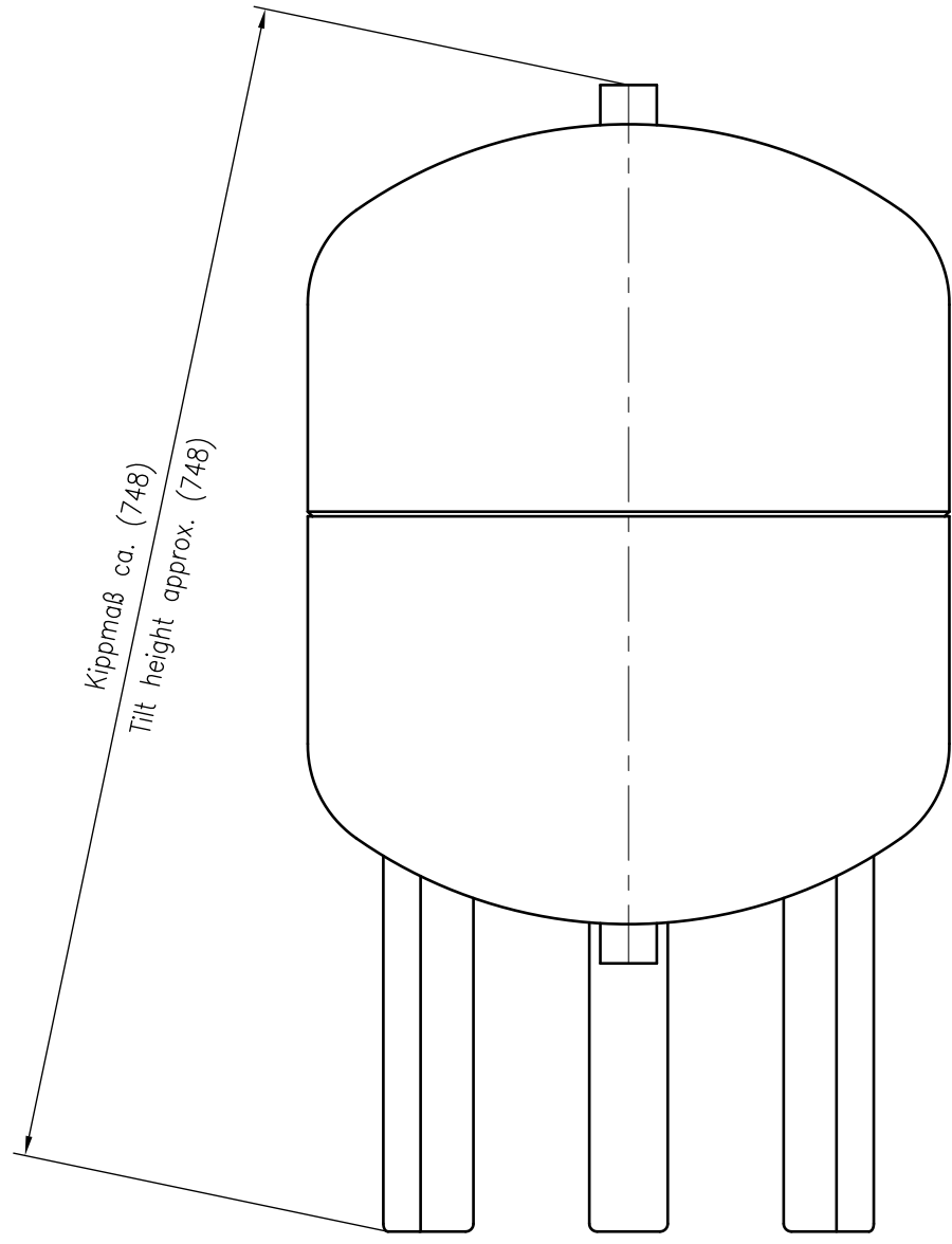
Side view
