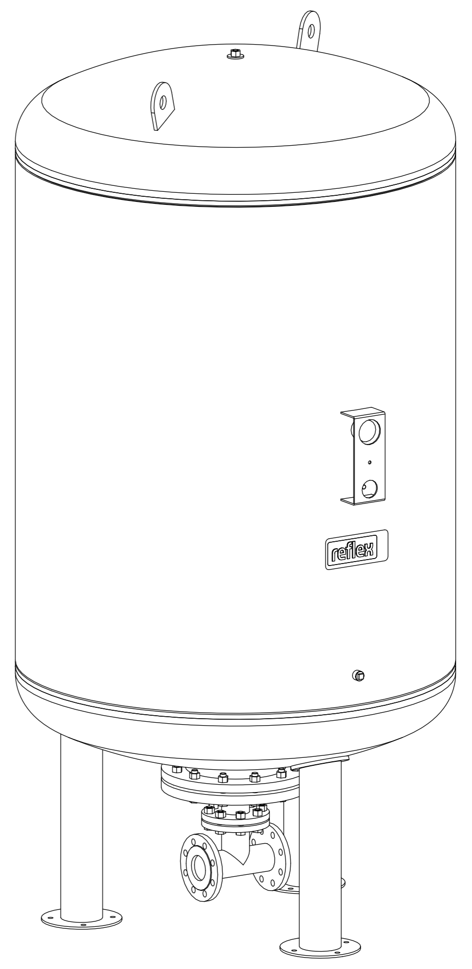
Isometric view
