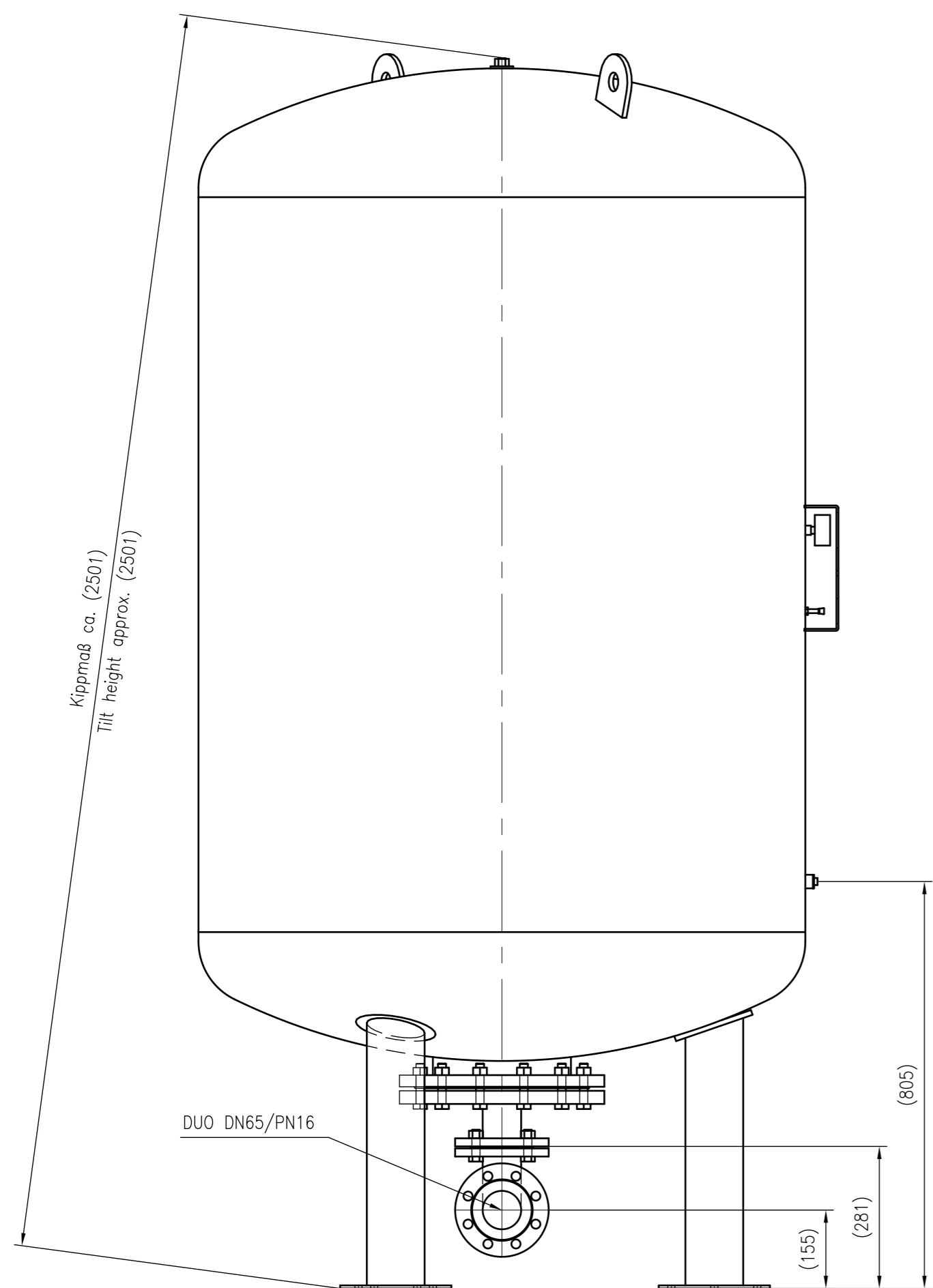
Side view
