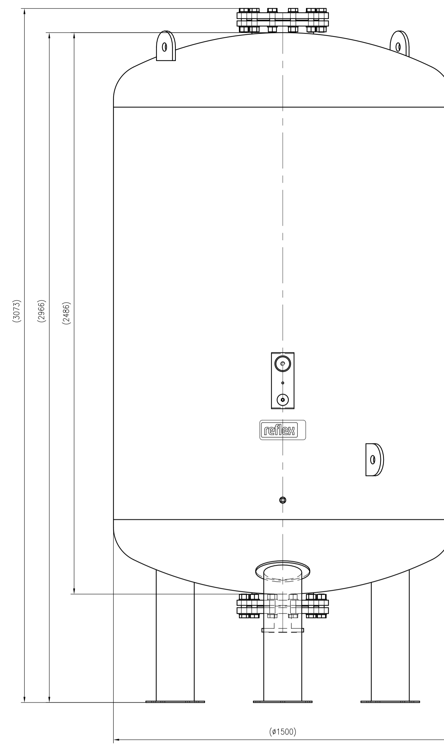
Front view
