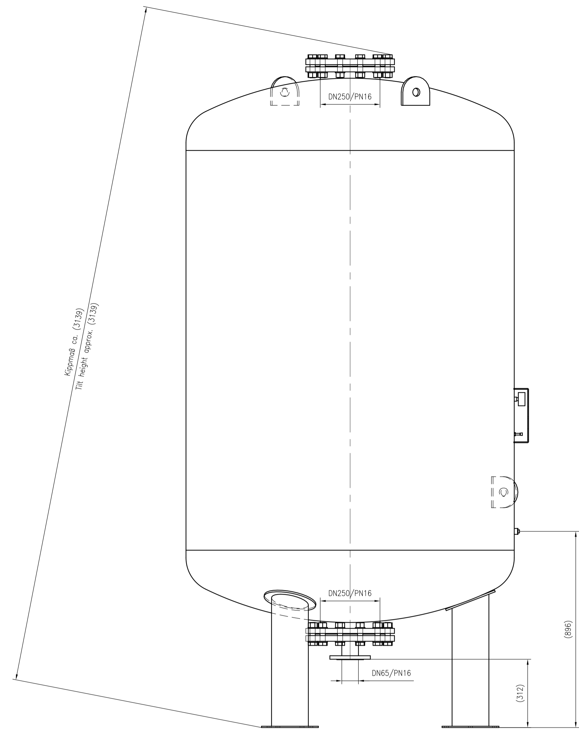
Side view
