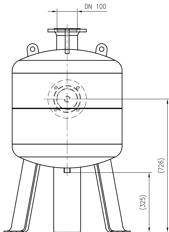
Side view
