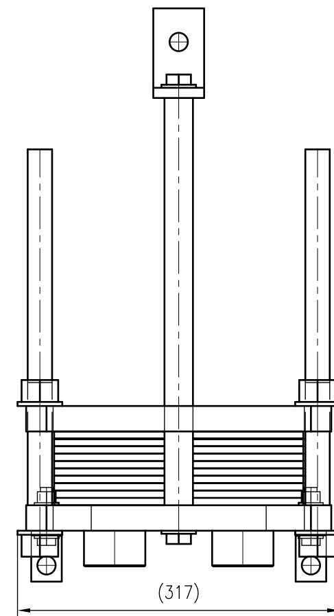
Top view
