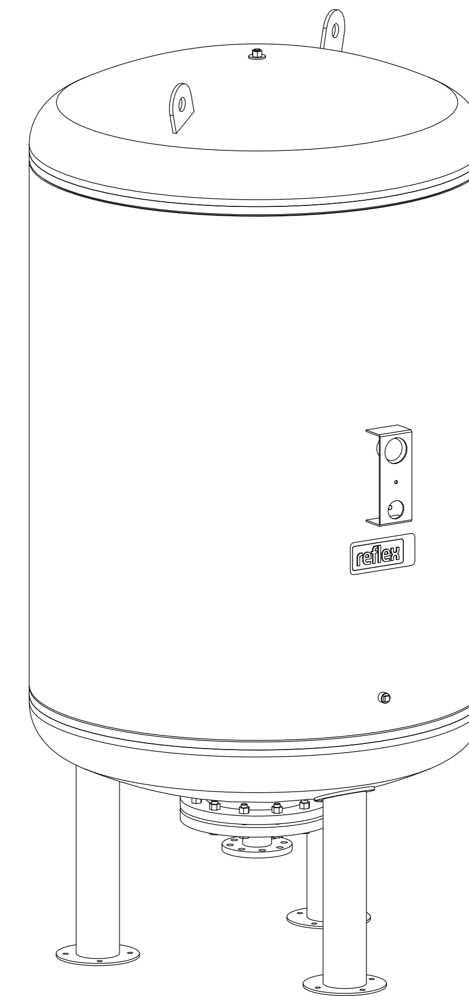
Isometric view
