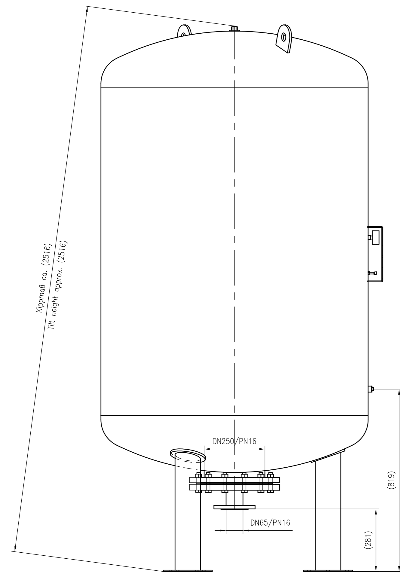
Side view
