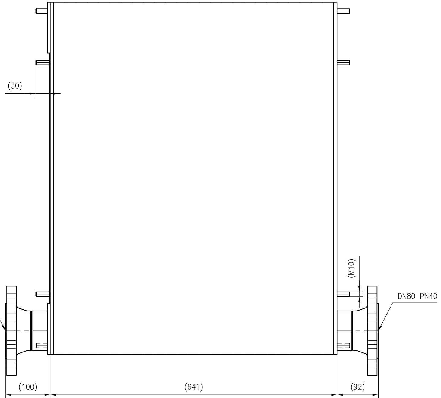
Side view
