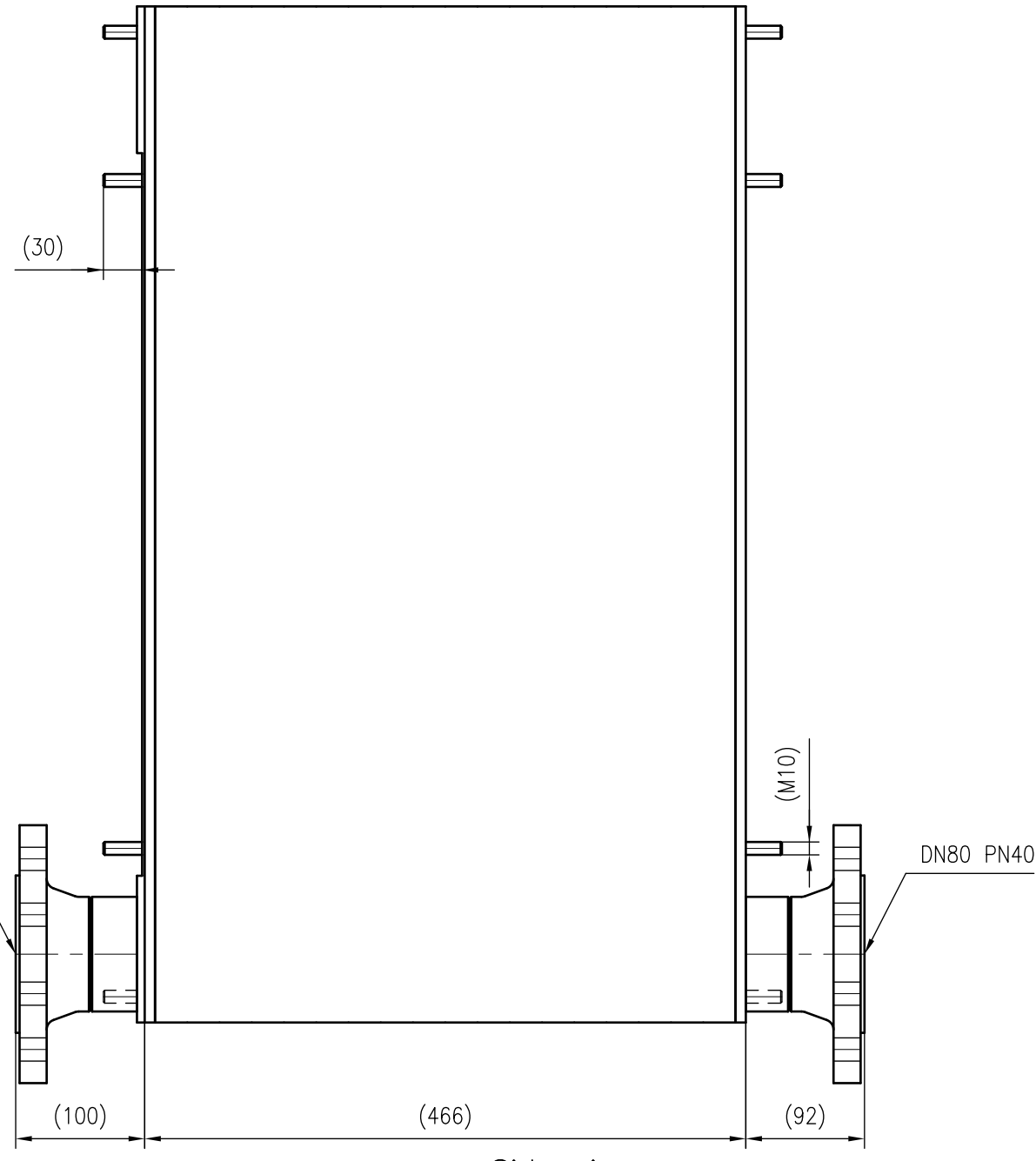
Side view
