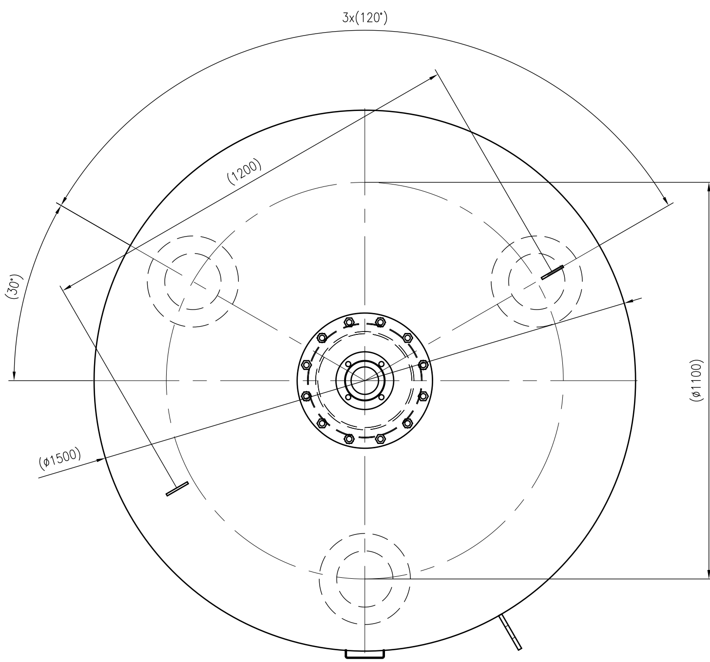
Top view
