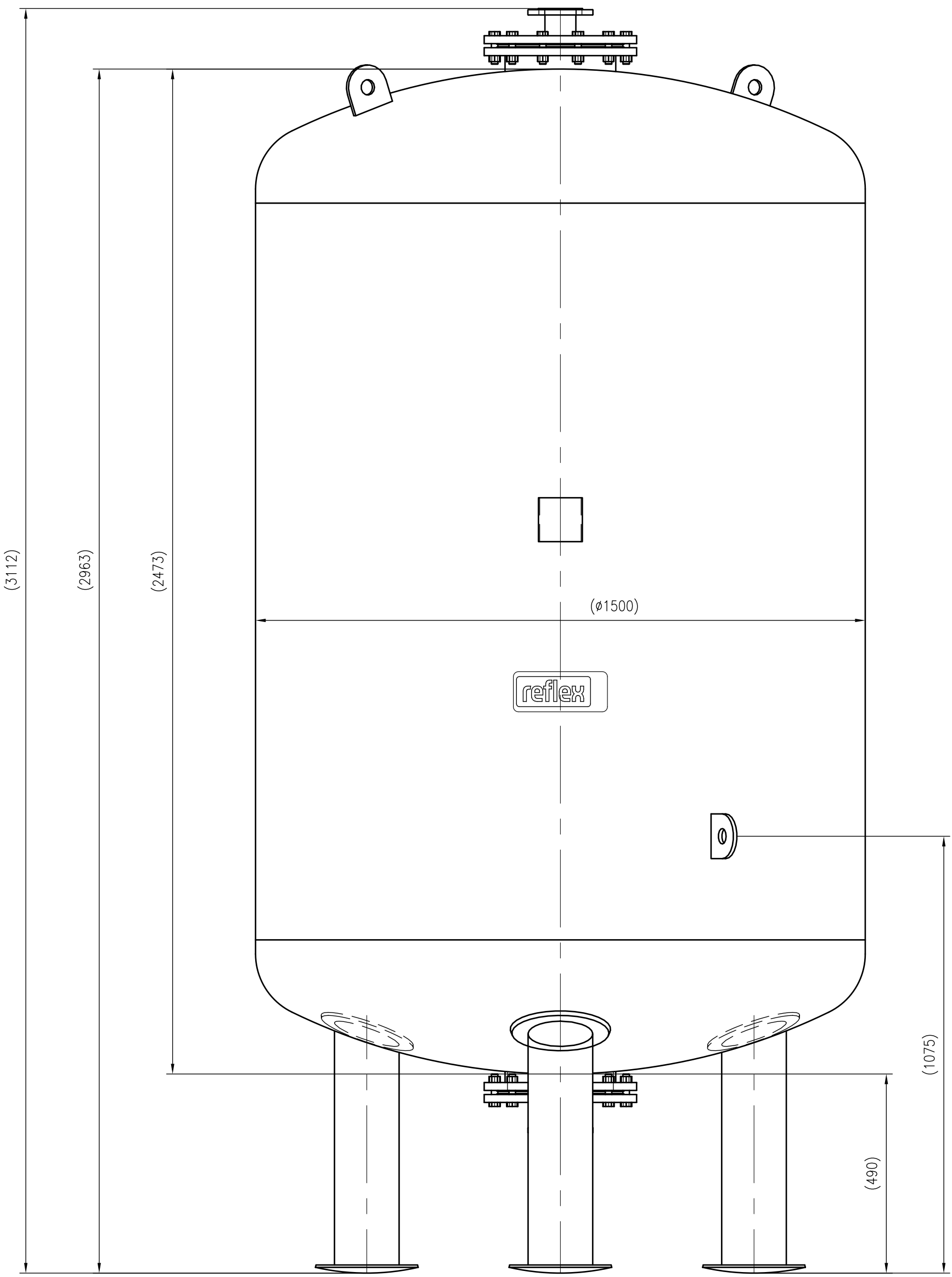
Front view
