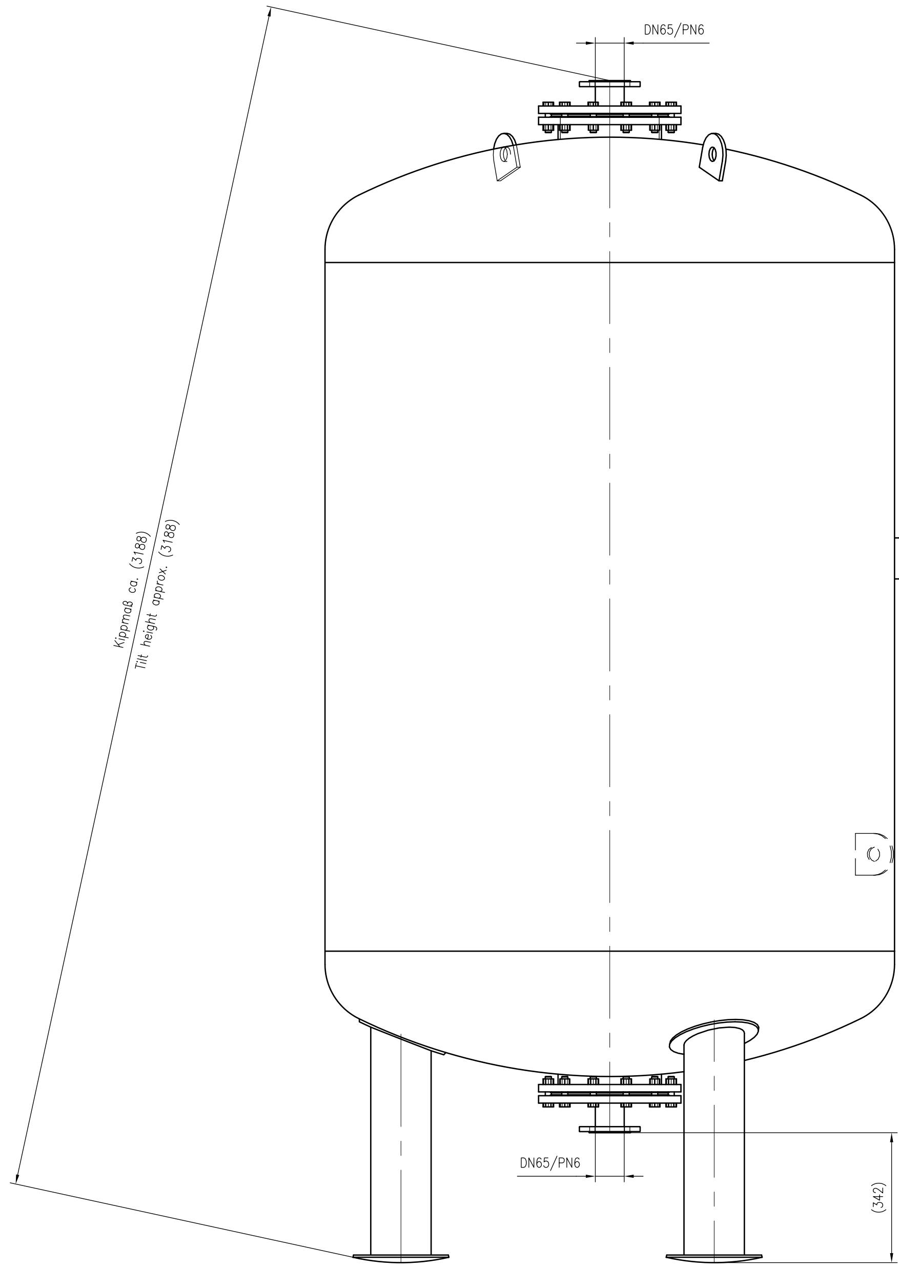
Side view
