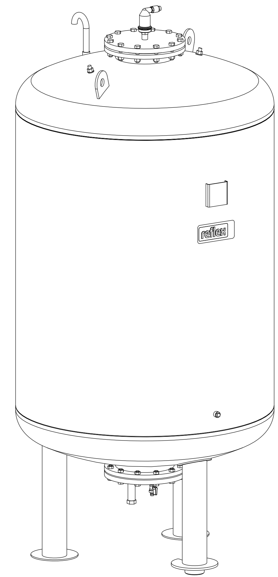
Isometric view
