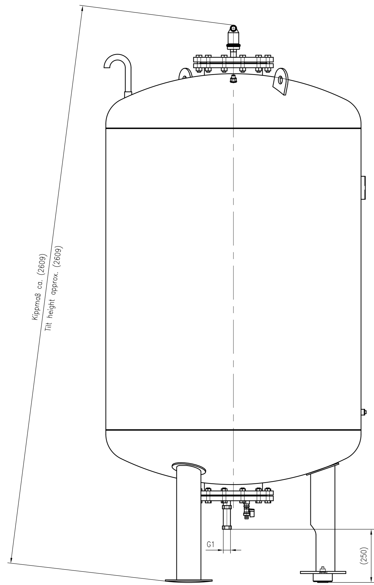
Side view
