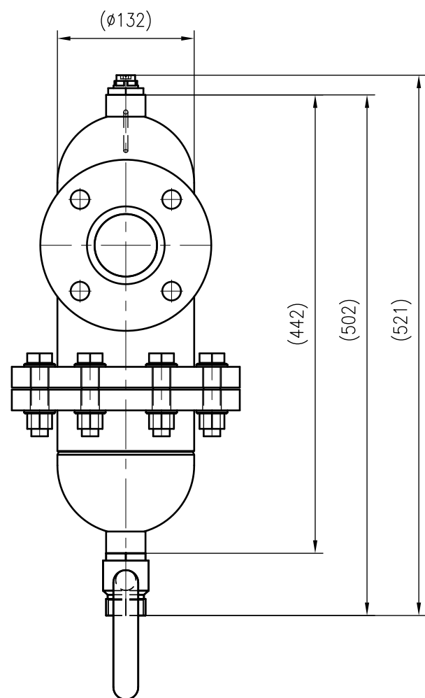
Side view
