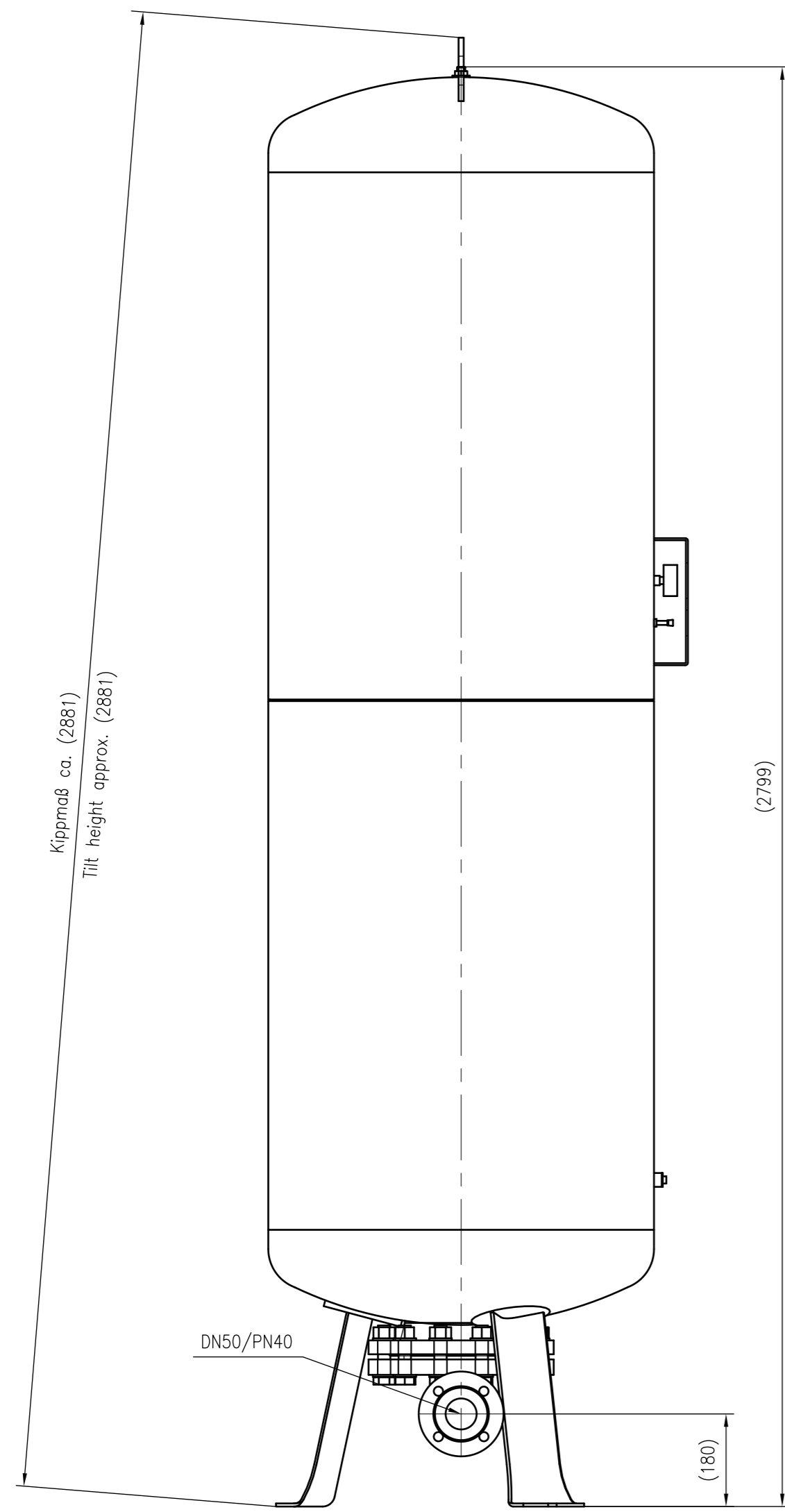
Side view
