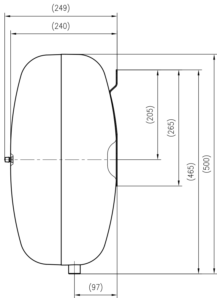
Side view
