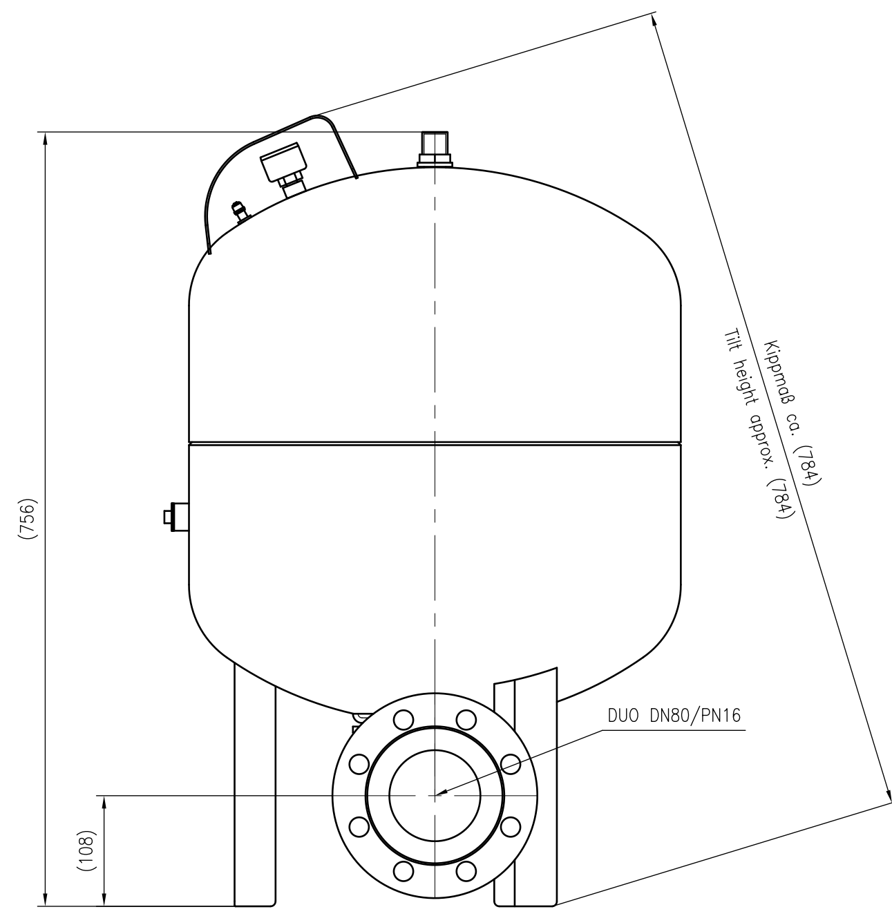
Side view
