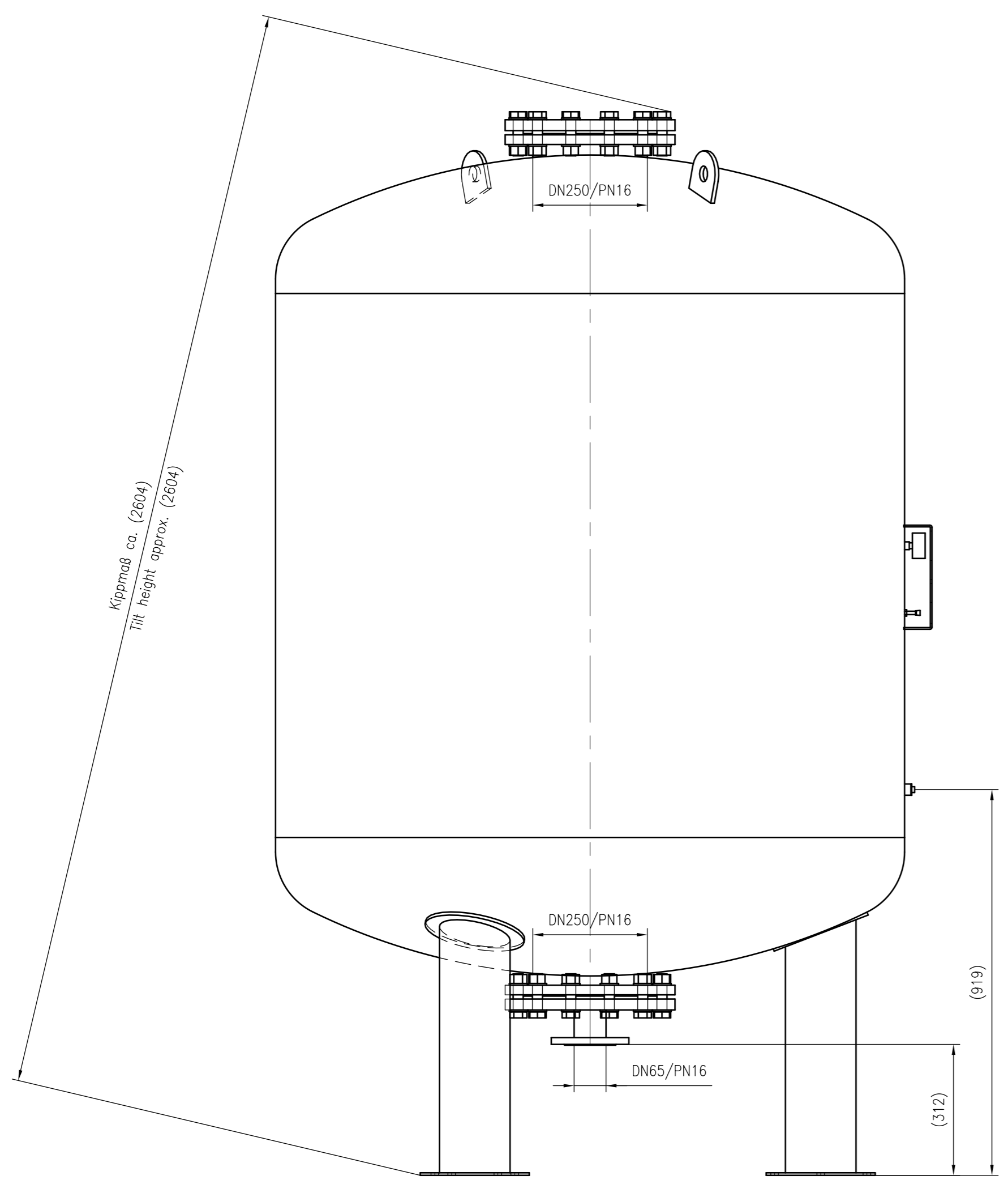
Side view
