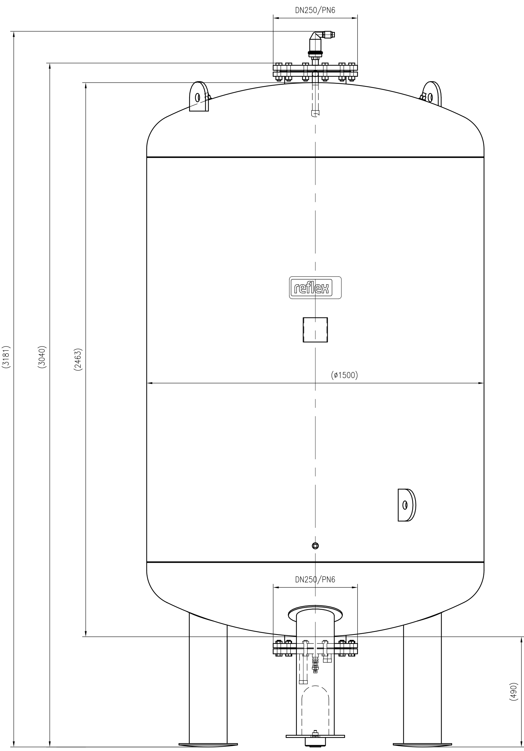
Front view
