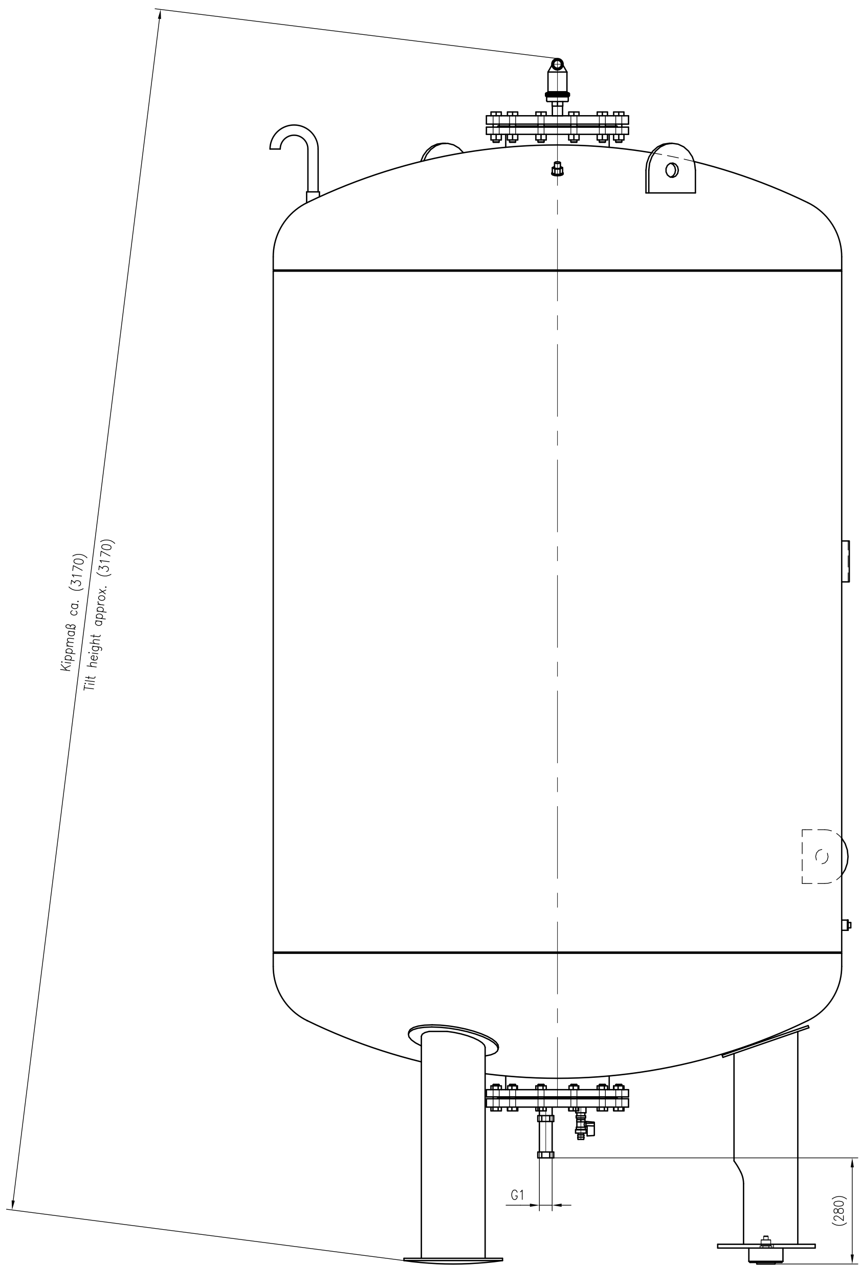
Side view
