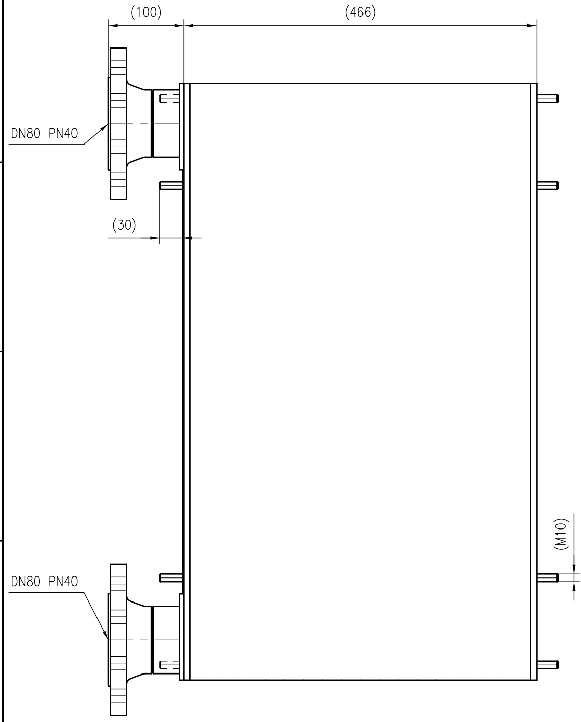
Side view
