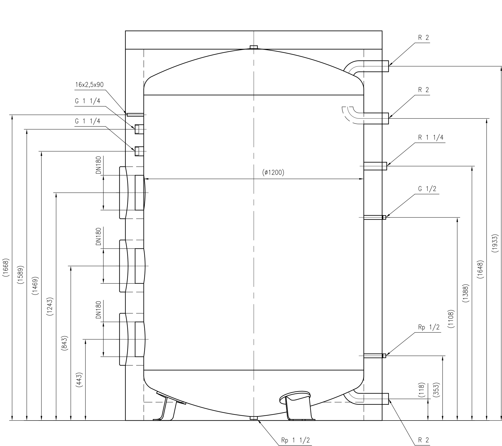
Side view
