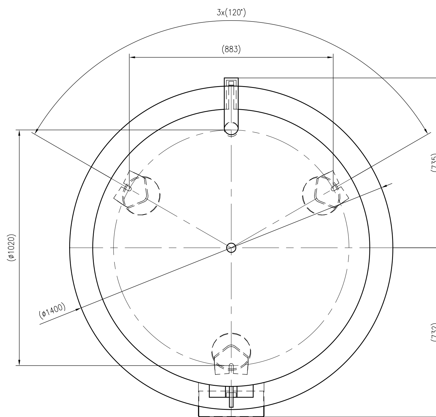
Top view
