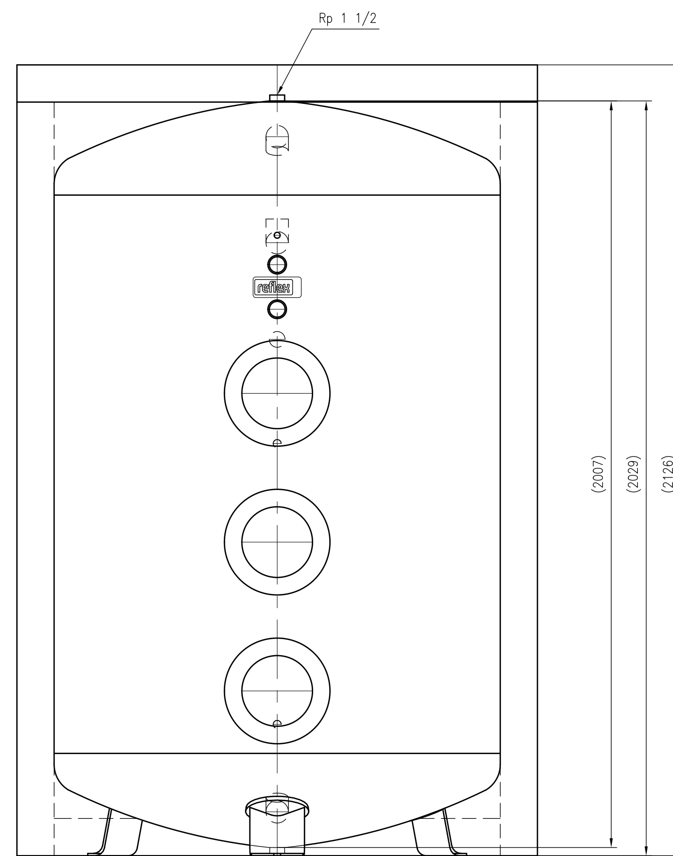
Front view
