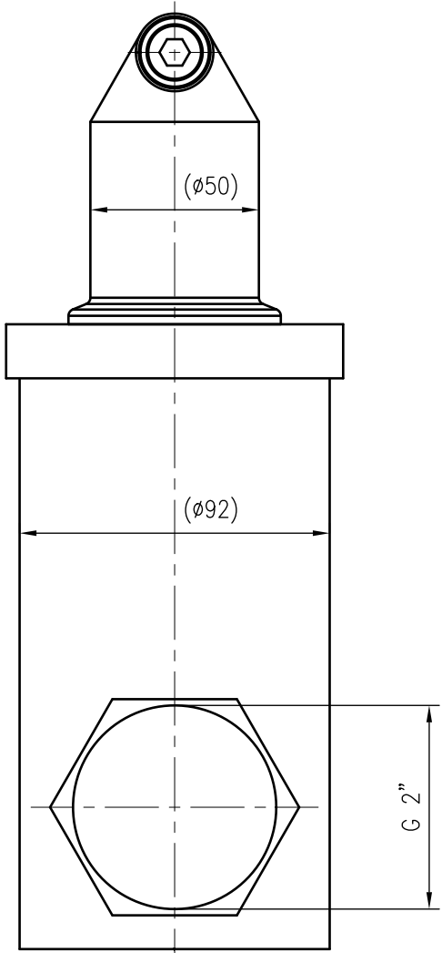
Side view
