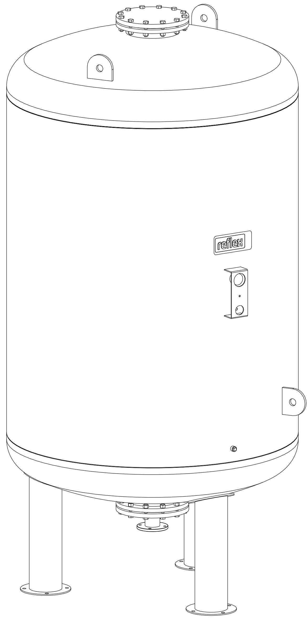
Isometric view
