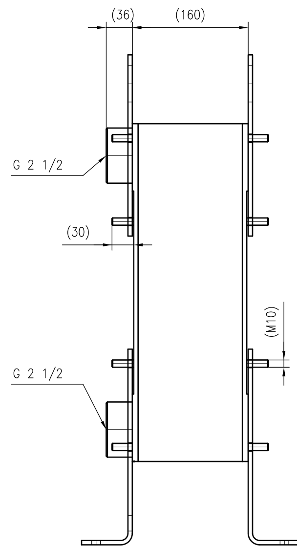
Side view
