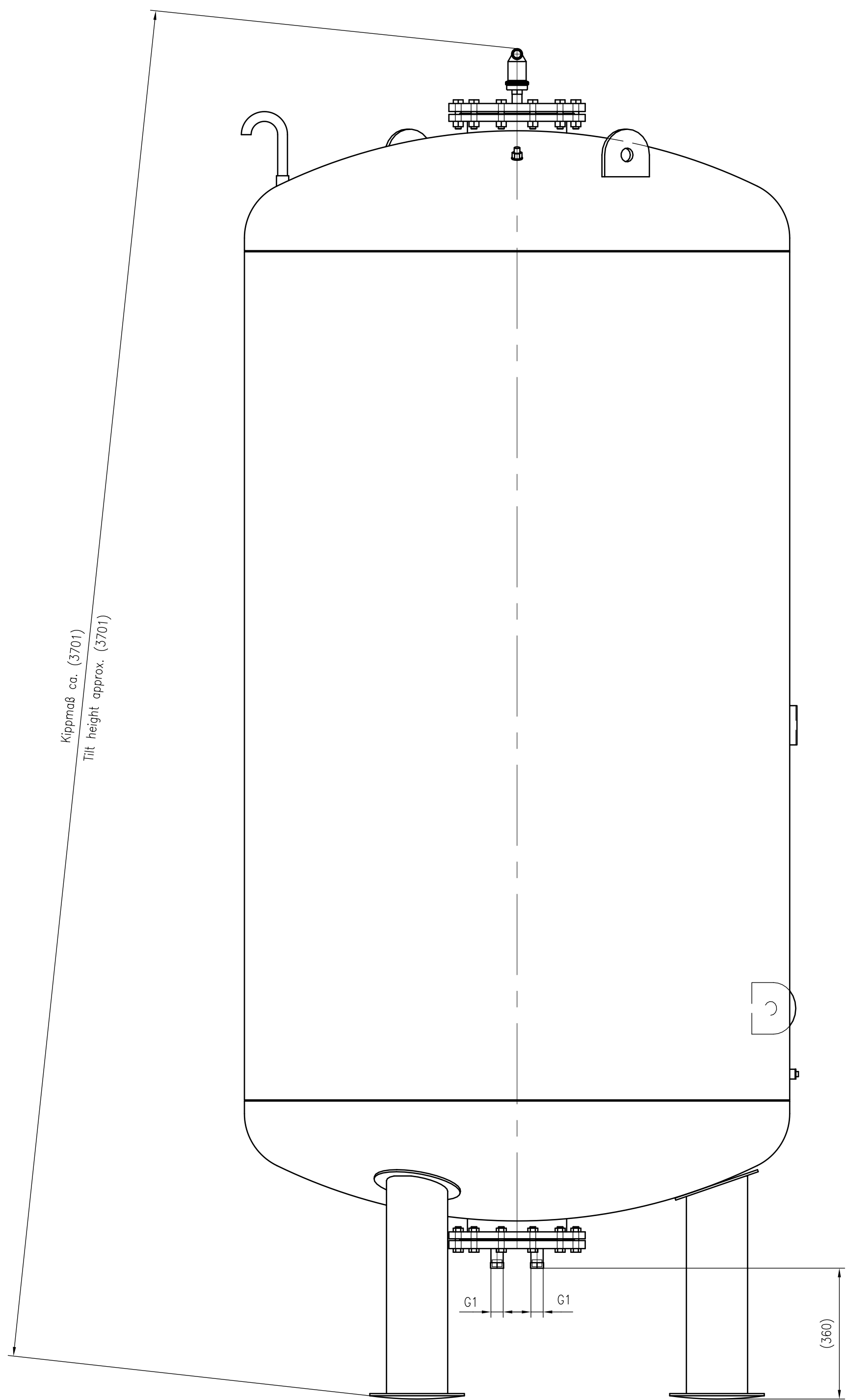
Side view
