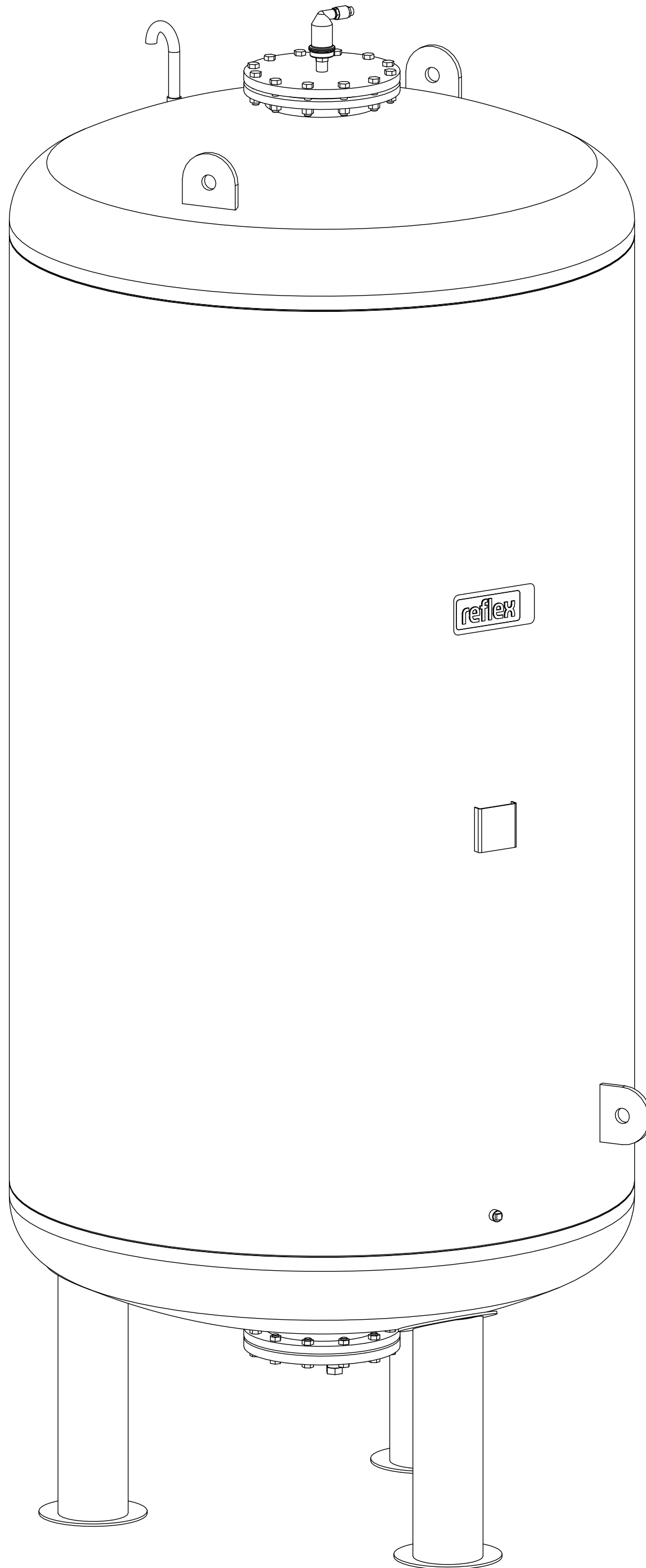
Isometric view
