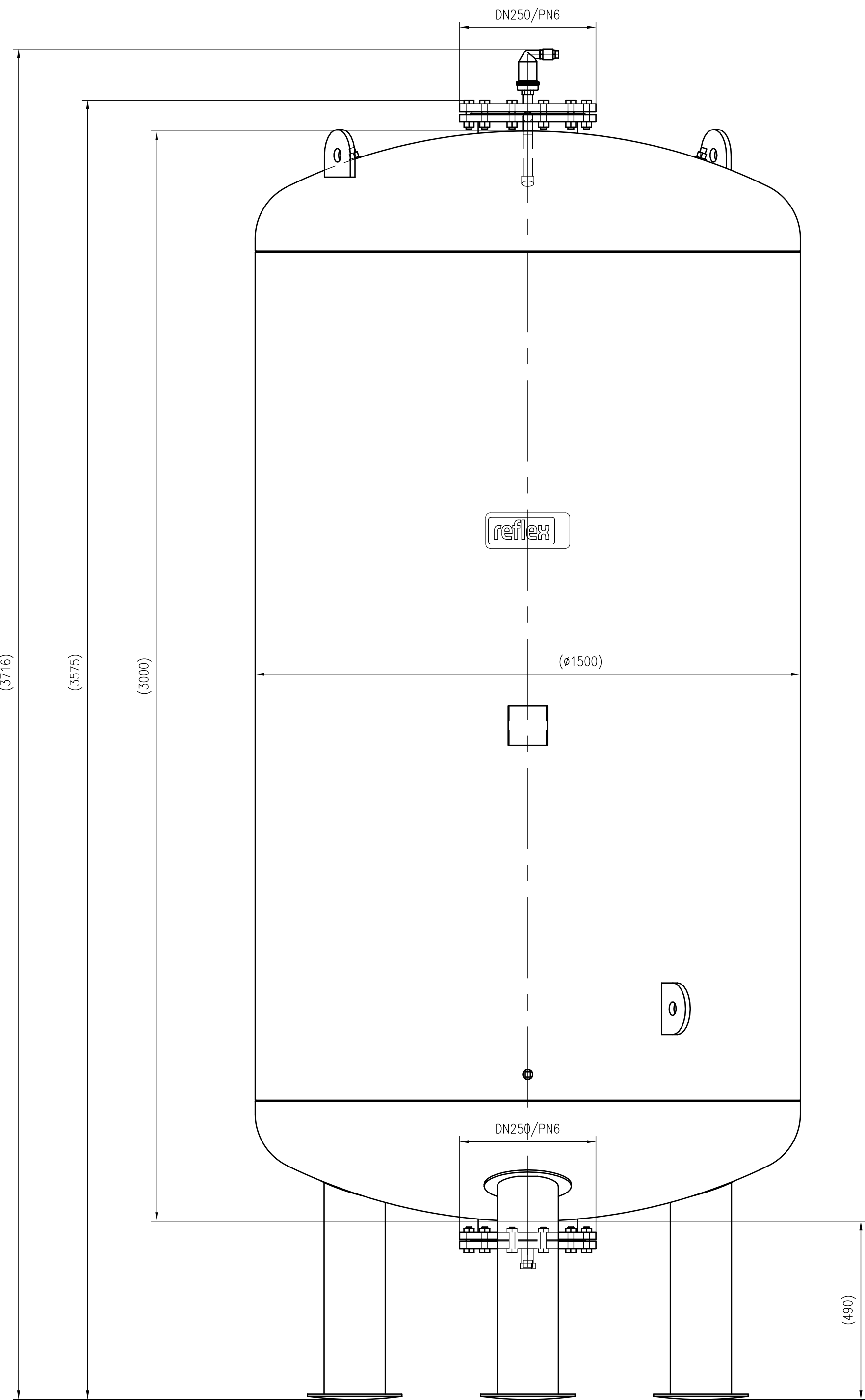
Front view
