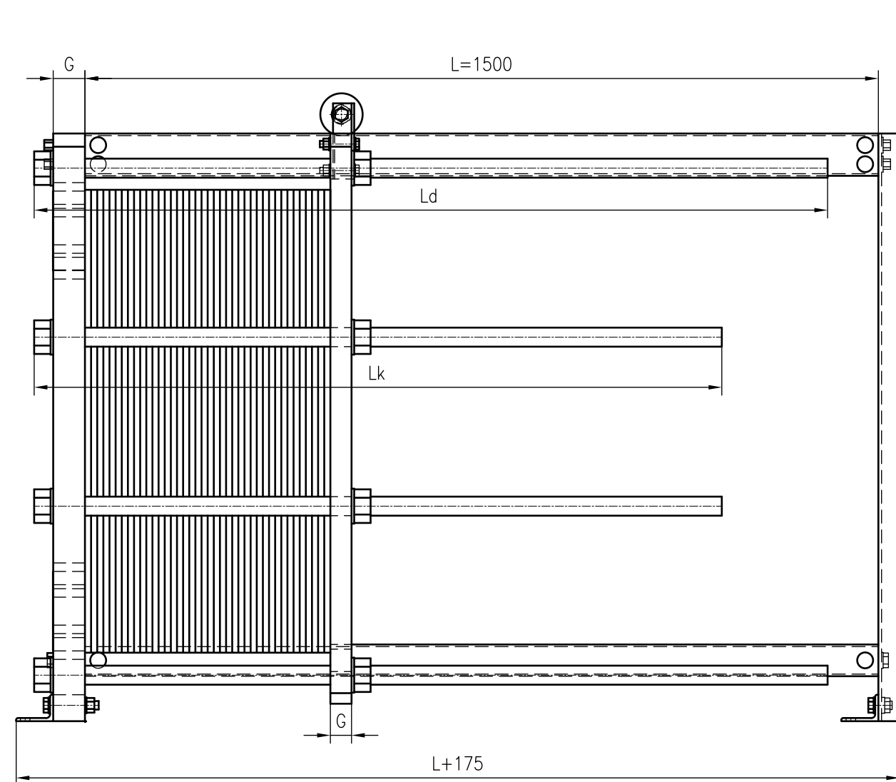
Side view
