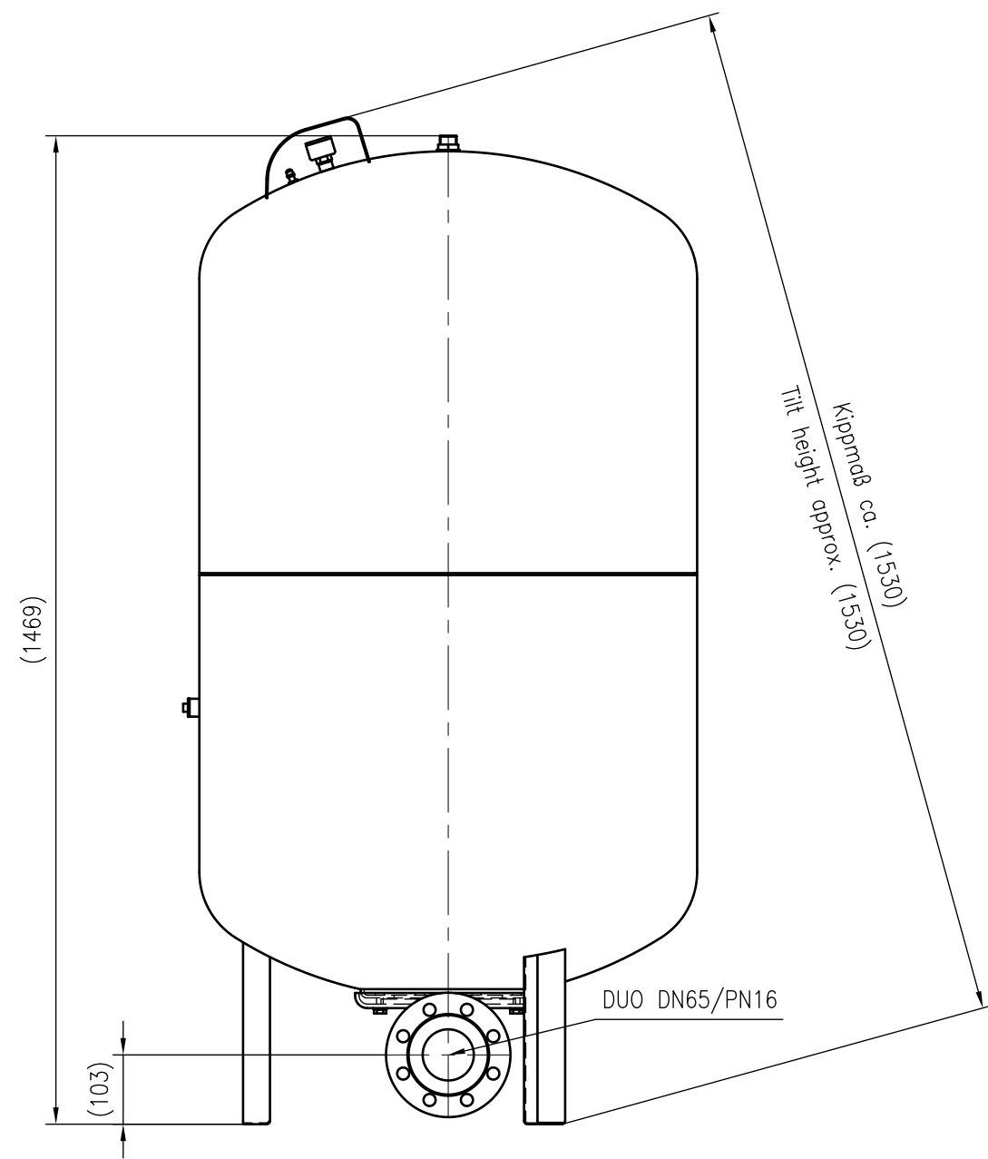
Side view
